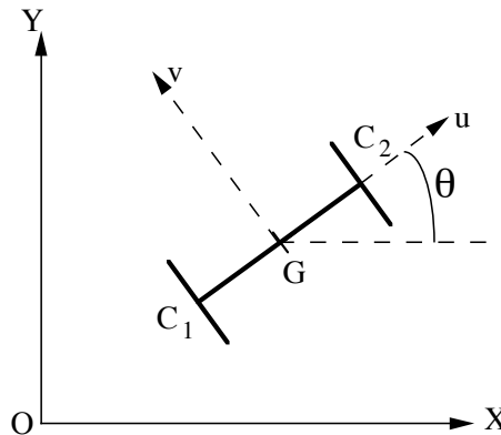
Figure 3.13: Essieu mobile sans glissement.
