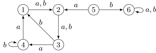
Fig. 3. The cycle 1 \xrightarrow{a} 2 \xrightarrow{a} 3 \xrightarrow{b} 1 is with external exit; the cycle 1 \xrightarrow{a} 2 \xrightarrow{a} 3 \xrightarrow{a} 4 \xrightarrow{a} 1 is with internal exit; and the cycle 6 \xrightarrow{a} 6 is without exit.
