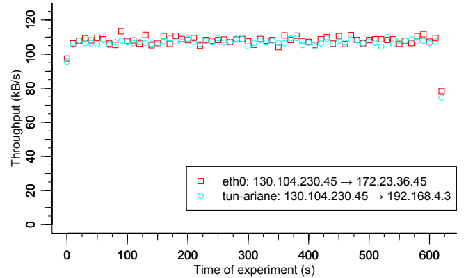
Fig. 6. Download using MPTCP and traffic control
