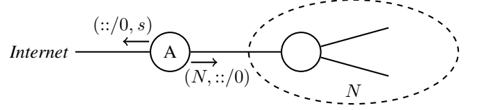
Fig. 3. A stub network behind a source-specific router
