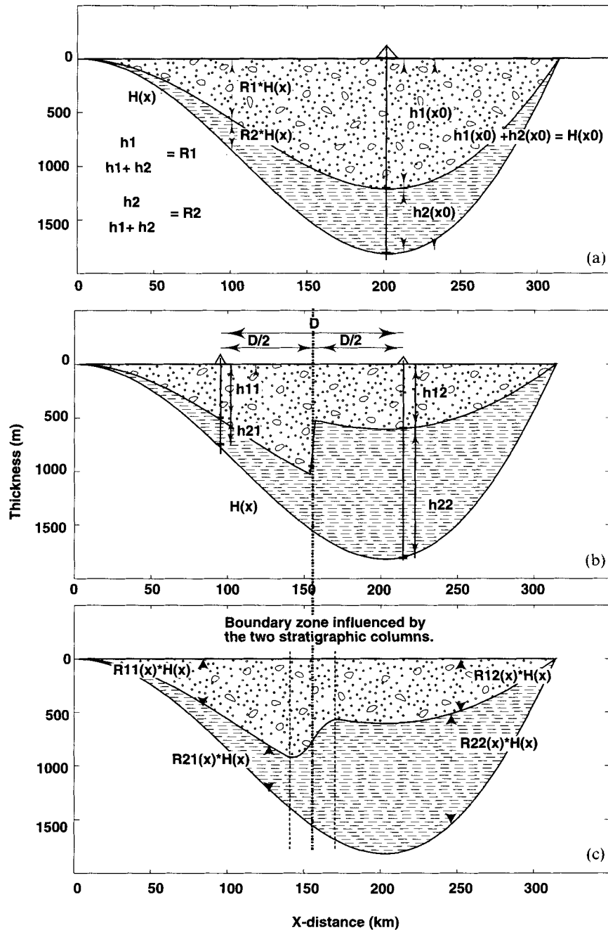
Figure 3. (a) 2-D reconstruction of two sedimentary layers from one isopach and one drill hole. (b), (c) Same as in (a) for one isopach and two drill holes, with smoothing of the transition zone. Variables are defined in the text.
