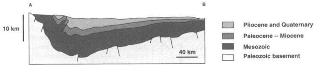
Figure 6. Simplified cross-section of Dzungar Basin from Peng & Guojun (1989) and Avouac (1991). See Fig. 1 for location of section.
