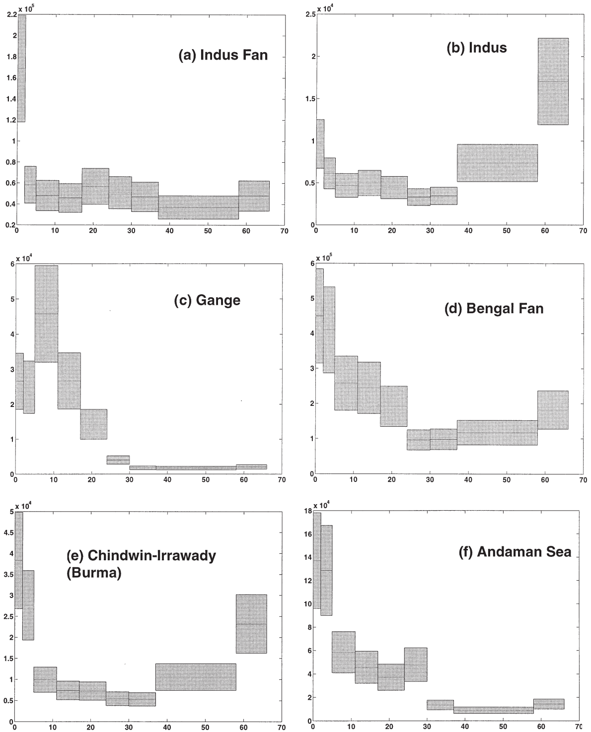
Figure 17. Average SPAR integrated over each major depositional area of reconstruction. x -axis: age in Ma; y -axis: rates in km 3 yr -1 . Grey-shaded boxes represent calculation uncertainty.
