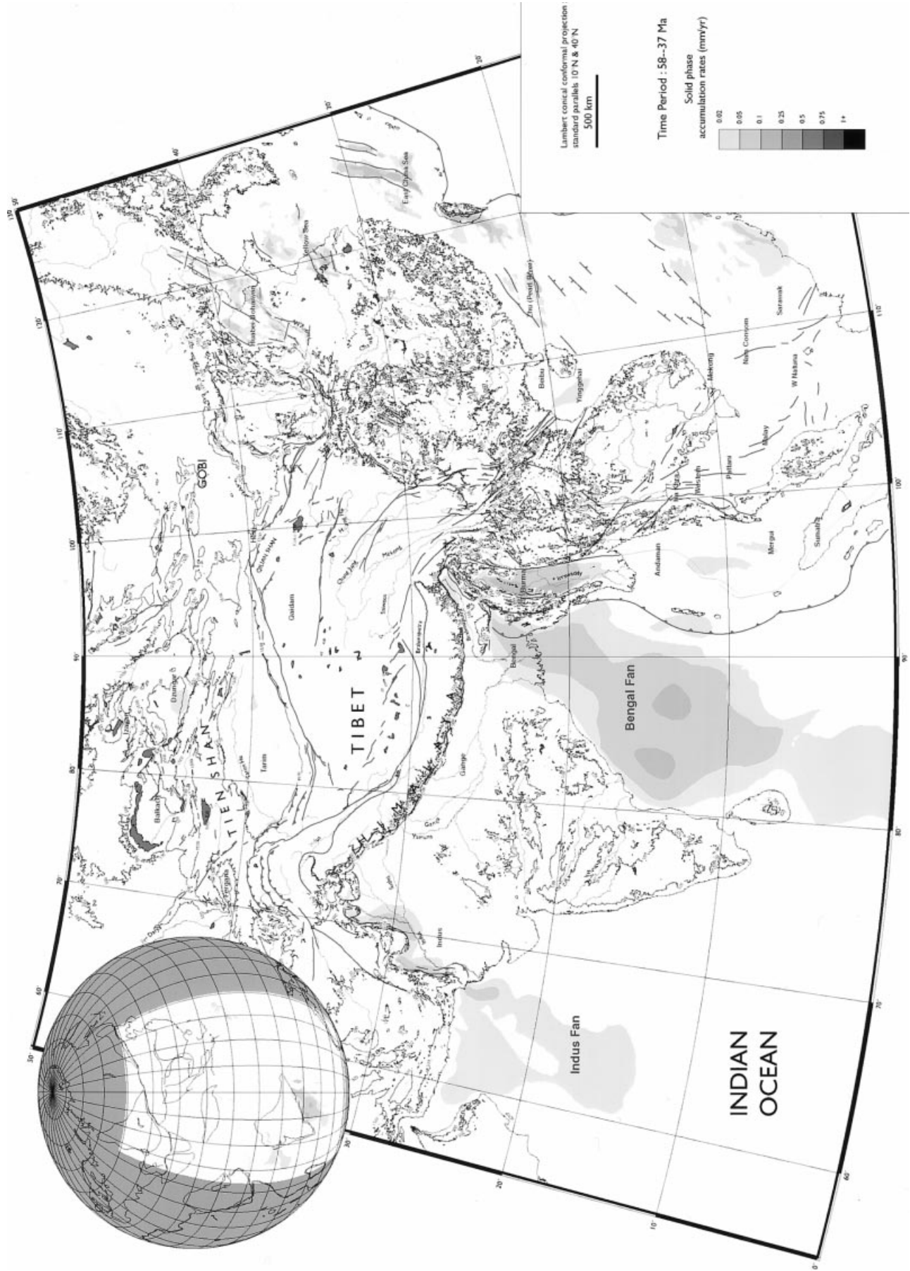
Figure 7. As Fig. 6 for the Eocene (~58–37 Ma).
