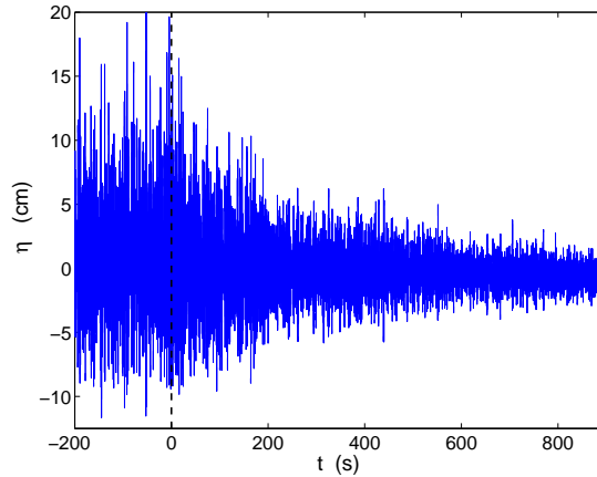
Figure 10: Decay of wave amplitude \eta(t) as a function of time for the reflecting boundary condition. Forcing is working for t < 0 and is stopped at t = 0 . Initial forcing conditions: FRN forcing with a narrow bandwidth ( f_m = 1.15 Hz, \Delta f = 0.3 Hz, \sigma_\eta = 4.6 cm).
