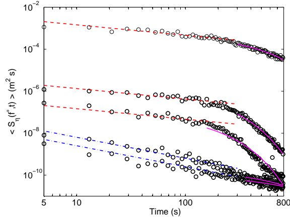
Figure 13: Temporal evolution of the wave spectrum \langle S_\eta(f^*, t) \rangle for Fourier components f^* = 1.2, 4.4, 8.3, 18.1, and 28.8 Hz (from top to bottom). Red dashed lines: t^{-1/2} law predicted for 4-wave interactions (gravity). Blue dot-dashed lines: t^{-1} law predicted for 3-wave interactions (capillary). Solid lines: exponential decay e^{-t/\tau_d(f^*)} as expected for a viscous damping, with \tau_d(f^*) the damping time. Closed basin.
