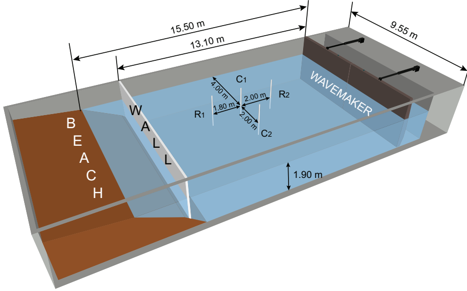
Figure 1: Sketch of the wave basin. The wavemaker is located on a side wall. The boundary opposed to the wavemaker is either a beach or a removable wall. The location of the array of probes is visible: capacitive probes C_1 and C_2 , and resistive ones R_1 and R_2 .
