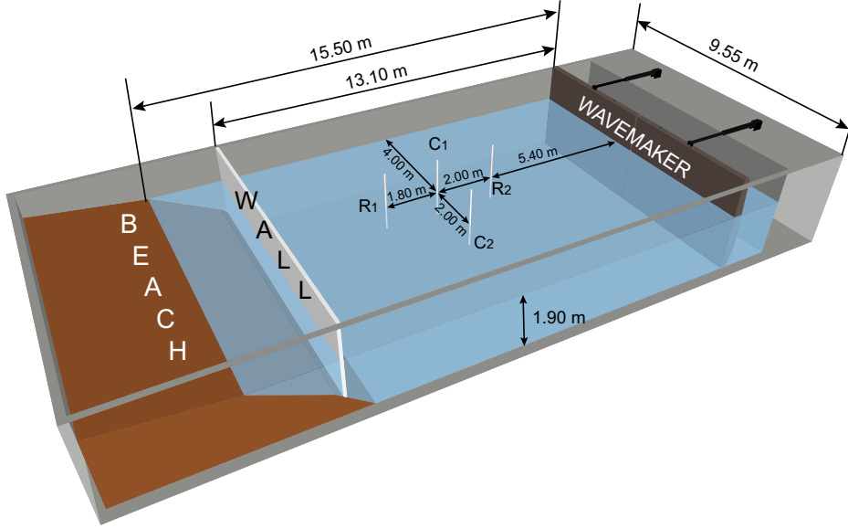
Figure 1: Sketch of the wave basin. The wavemaker is located . The boundary oppo the wavemaker is either a beach or a removable wall. The location of the array of probes is visible: capacitive probes C_1 and C_2 , and resistive ones R_1 and R_2 .
