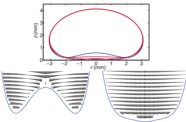
FIG. 13. (Color online) Drop contours during the final stages of the simulation in an unstable scenario (see Fig. 12). Blue contours are the two extremes, red lines are intermediate. The bottom two plots show the velocity profile inside the drop for the extremes. Note that the liquid velocities, and therefore the oscillations as well, are mainly in the vertical direction. Bo = 1 , Ca = 2.5 \times 10^{-4} , \Lambda = 8.2 \times 10^3 .
