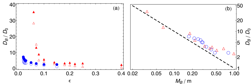
FIG. 10. (a) Plot of the diffusion coefficient D_B , normalized by the free particle diffusion coefficient D_0 = k_B T / m \gamma , as a function of the confinement \epsilon , for N = 32 and L = 60 mm (red triangles) and N = 64 and L = 120 mm (blue circles). The closed symbols correspond to the diffusion coefficients deduced from the long-time MSD and the open symbols correspond to the calculated diffusion coefficients k_B T / M_B \gamma , where the mass M_B is given by (10). (b) A log-log plot of D_B / D_0 as a function of the dimensionless mass M_B / m of the quasiparticle. The dashed line is the theoretical expectation of slope -1 .
