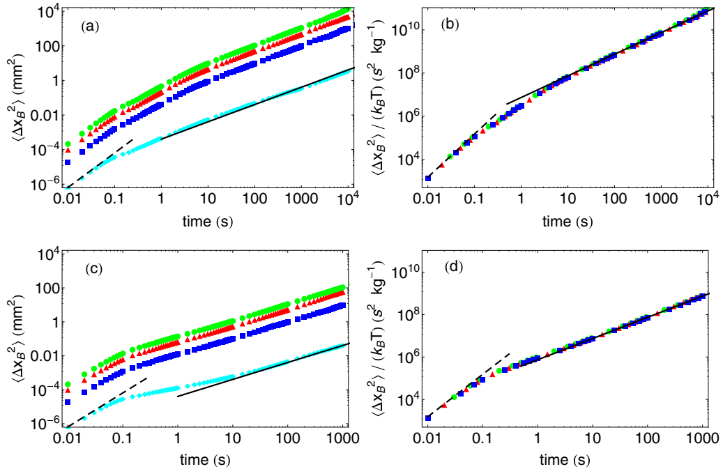
FIG. 6. (a) and (c) Plots of the bubble MSD (logarithmic scale, in mm ^2 ) as a function of time (logarithmic scale, in s) for N = 32 particles in a cell of length L = 60 mm and \epsilon = 0.08 . The temperatures are T = 10^9 K (blue squares), T = 5 \times 10^9 K (red triangles), and T = 10^{10} K (green circles). The damping constant is (a) \gamma = 1 s ^{-1} and (c) \gamma = 10 s ^{-1} . For the sake of comparison, the longitudinal MSDs of a typical particle in the system with temperature T = 10^9 K are shown as cyan diamonds. The dashed black lines correspond to the ballistic regime and the solid black lines to the diffusive regimes for a single particle in the chain [30]. (b) and (d) Plots of \langle \Delta x_B^2(t) \rangle / k_B T (logarithmic scale, in s ^2 kg ^{-1} ) as a function of time (logarithmic scale, in s) for (b) \gamma = 1 s ^{-1} and (d) \gamma = 10 s ^{-1} . The solid black line is the free diffusion of a bubble of mass M_B defined in Eq. (10) and the dashed black line is the ballistic regime of Eq. (15), without any fitting parameter.
