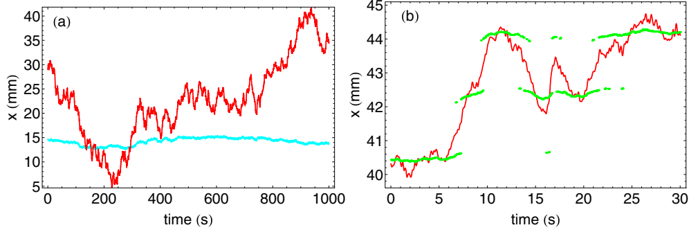
FIG. 5. Plot of the longitudinal displacements (in mm) as a function of time (in s), for a system of N = 32 particles, L = 60 mm, at T = 5 \times 10^9 K, \gamma = 1 s ^{-1} , and \epsilon = 0.08 . (a) Typical trajectory of a bubble, measured by x_B(t) [red (dark gray) solid line], and longitudinal motion of a typical particle [cyan (light gray) solid line]. (b) Zoom in on the bubble trajectory (red solid line) [note the scale difference from (a)] and instantaneous position of the particle with maximum transverse displacement (green dots).
