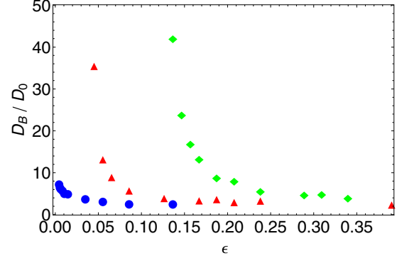
FIG. 8. Plot of the diffusion coefficient D_B extracted from the long-time behavior of the bubble MSD, normalized by the diffusion coefficient of a free single particle D_0 = k_B T / m \gamma , as a function of the confinement \epsilon . We show data for N = 16 and L = 30 mm (green diamonds), N = 32 and L = 60 mm (red triangles), and N = 64 and L = 120 mm (blue circles).
