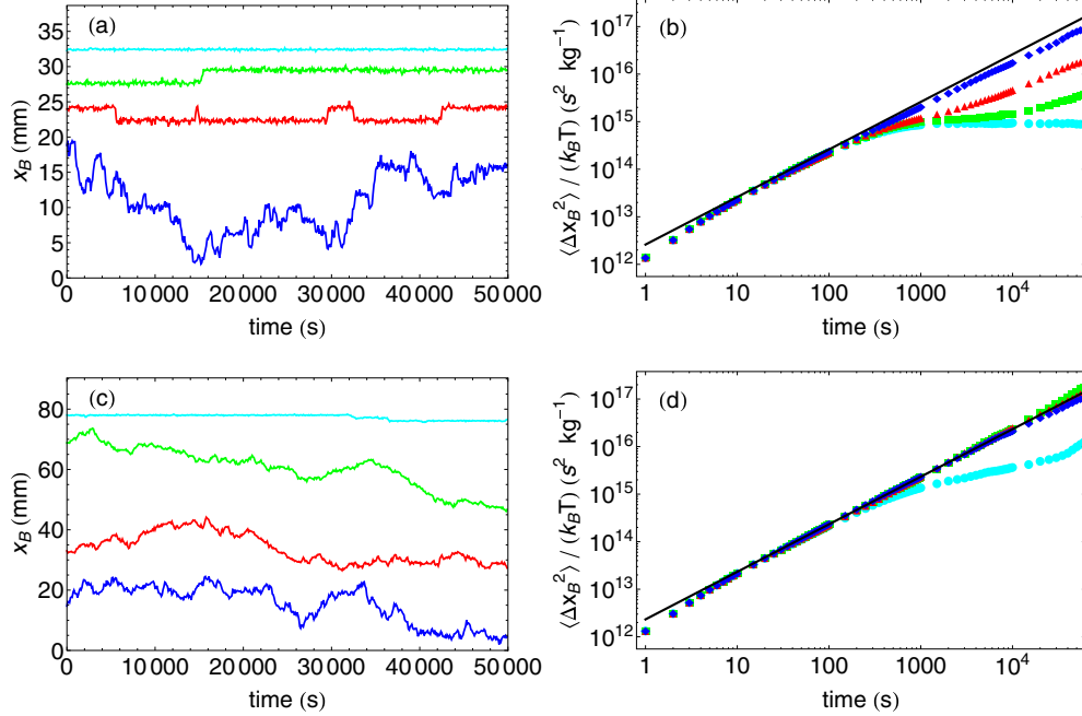
FIG. 11. (a) and (c) Plots of the longitudinal bubble position x_B (in mm) as a function of time (in s), for a system of N = 64 particles in a cell of L = 120 mm with \gamma = 1 s -1 . (a) and (b) The confinement is \epsilon_t = 0.085 and \Delta E(\epsilon_t) = 7.9 \times 10^{-10} nJ. (c) and (d) The confinement is \epsilon_b = 0.093 and \Delta E(\epsilon_b) = 1.0 \times 10^{-10} nJ. The temperatures are T = 10^6 K (cyan circles), T = 5 \times 10^6 K (green squares), T = 7 \times 10^6 K (red triangles), and 2 \times 10^7 K (blue diamonds). (b) and (d) Plots of the corresponding MSD \langle \Delta x_B^2(t) \rangle / k_B T (logarithmic scale, in s 2 kg -1 ) as a function of time (logarithmic scale, in s).
