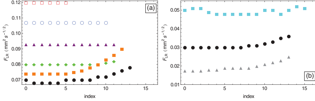
FIG. 6. (Color online) Mobility ( \text{mm}^2\text{s}^{-1/2} ) as a function of the particle index for 33 particles: (a) \gamma = 1 \text{ s}^{-1} . HW confinement, \lambda_w = 0.48 \text{ mm} , E_w/E_0 = 0.0095 (red open squares); SW confinement, \lambda_w = 0.48 \text{ mm} , E_w/E_0 = 0.1 (blue circles); LR confinement, E_w/E_0 = 0.1 , \lambda_w = 4 \text{ mm} (magenta triangles), 7 \text{ mm} (green diamonds), 11 \text{ mm} (orange squares), 15 \text{ mm} (black dots). (b) \gamma = 60 \text{ s}^{-1} . LR confinement, \lambda_w = 15 \text{ mm} , E_w/E_0 = 0.001 (red diamonds), 0.05 (pink circles), 0.1 (black dots).
