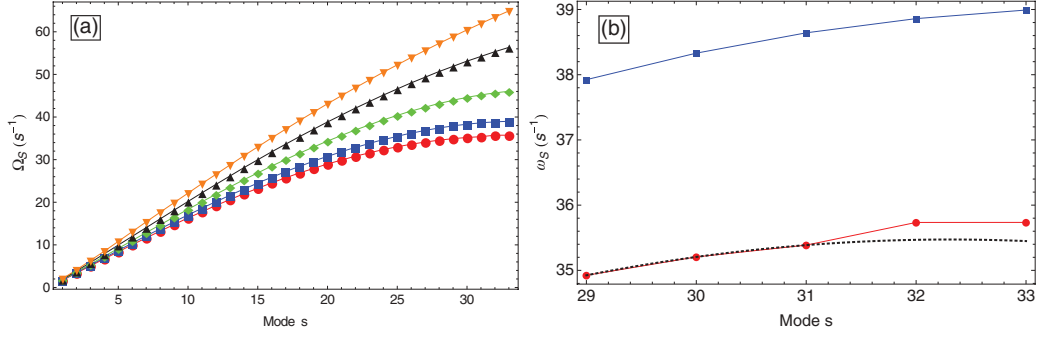
FIG. 10. (Color online) (a) Dispersion relation of the normal modes for a system of 33 particles. HW confinement, \lambda_w = 0.48 mm, E_w/E_0 = 0.0095 (red dots); SW confinement, \lambda_w = 1 mm, E_w/E_0 = 0.1 (blue squares); LR confinement, E_w/E_0 = 0.1 , \lambda_w = 4 mm (green diamonds), 11 mm (black triangles up), 30 mm (orange triangles down). (b) Focus on the dispersion equation of the highest frequencies for the HW (red dots) and the SW (blue squares) cases: for HW the two highest frequencies are associated to localized modes. The dotted line is a guide for the eyes.
