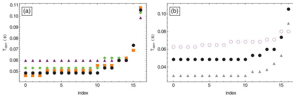
FIG. 7. (Color online) Correlation time t_{\text{corr}} (s) as a function of the particle index for 33 particles, \gamma = 1 \text{ s}^{-1} and a LR confinement. (a) E_w/E_0 = 0.1 , \lambda_w = 4 \text{ mm} (magenta triangles), 7 \text{ mm} (green diamonds), 11 \text{ mm} (black dots), 15 \text{ mm} (orange squares). (b) \lambda_w = 15 \text{ mm} , E_w/E_0 = 0.005 (pink circles), 0.1 (black dots), 0.5 (gray triangles).
