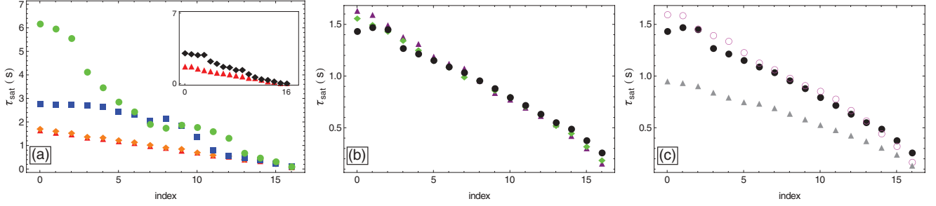
FIG. 8. (Color online) Saturation time t_{\text{sat}} (s) as a function of the particle index for 33 particles. (a) SW confinement, E_w/E_0 = 0.1 , \lambda_w = 1 mm: \gamma = 0.1 s ^{-1} (red triangles); 1 s ^{-1} (orange diamonds); 10 s ^{-1} (blue square); 20 s ^{-1} (green dots). Inset: Plot of t_{\text{sat}} in the HW case: \gamma = 1 s ^{-1} (red triangles); 10 s ^{-1} (black diamonds). (b) LR confinement, E_w/E_0 = 0.1 , \gamma = 1 s ^{-1} , \lambda_w = 4 mm (magenta triangles); 7 mm (green diamonds); 15 mm (black dots). (c) LR confinement with \gamma = 1 s ^{-1} , \lambda_w = 15 mm, E_w/E_0 = 0.05 (pink circles); 0.1 (black dots); 0.5 (gray triangles).
