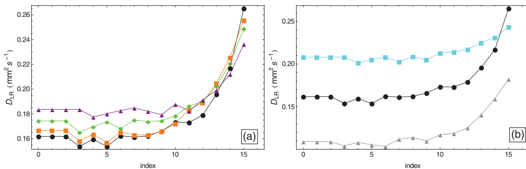
FIG. 16. (Color online) Plot of the theoretical diffusivities (in \text{mm}^2\text{s}^{-1} ) as a function of the particle index n . (a) E_w/E_0 = 0.1 , \lambda_w = 4 mm (magenta triangles), 7 mm (green diamonds), 11 mm (orange squares), and 30 mm (red dots). (b) \lambda_w = 15 mm, E_w/E_0 = 0.005 (cyan squares), 0.1 (black dots), and 0.5 (gray triangles). The mobilities are \sqrt{\gamma/3}D_{\text{LR}} .
