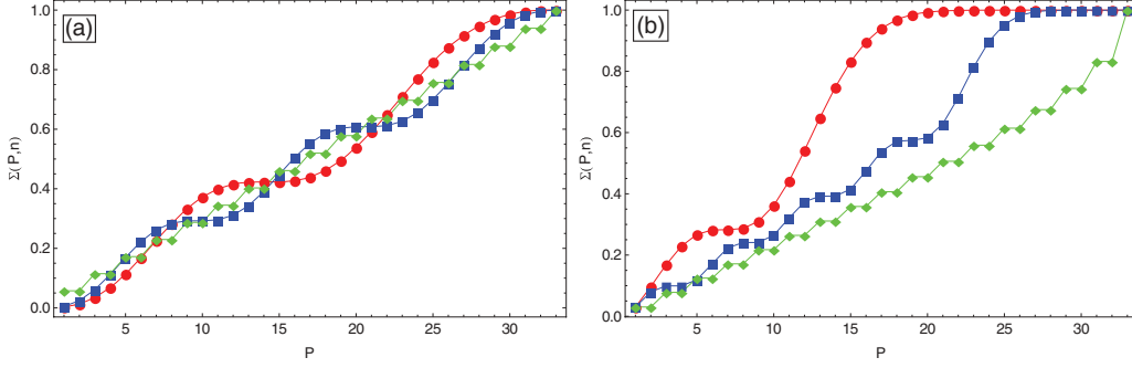
FIG. 14. (Color online) Plot of the partial sum \Sigma(P, n) as a function of P for particles n = \pm 15 (red dots), n = \pm 14 (blue squares), and n = 0 (green diamonds). (a) SW confining potential with \lambda_w = 1 mm and E_w/E_0 = 0.1 . (b) LR confining potential with \lambda_w = 30 mm and E_w/E_0 = 0.1 .
