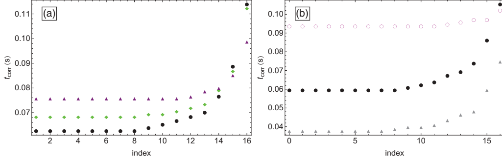
FIG. 17. (Color online) (a) Theoretical correlation times t_{\text{corr}} (s) as a function of the particle index n . (a) E_w/E_0 = 0.1 ; \lambda_w = 4 mm (magenta triangles), 7 mm (green diamonds), 15 mm (black dots). (b) \lambda_w = 15 mm; E_w/E_0 = 0.005 (magenta circles), 0.1 (black dots), and 0.5 (gray triangles).
