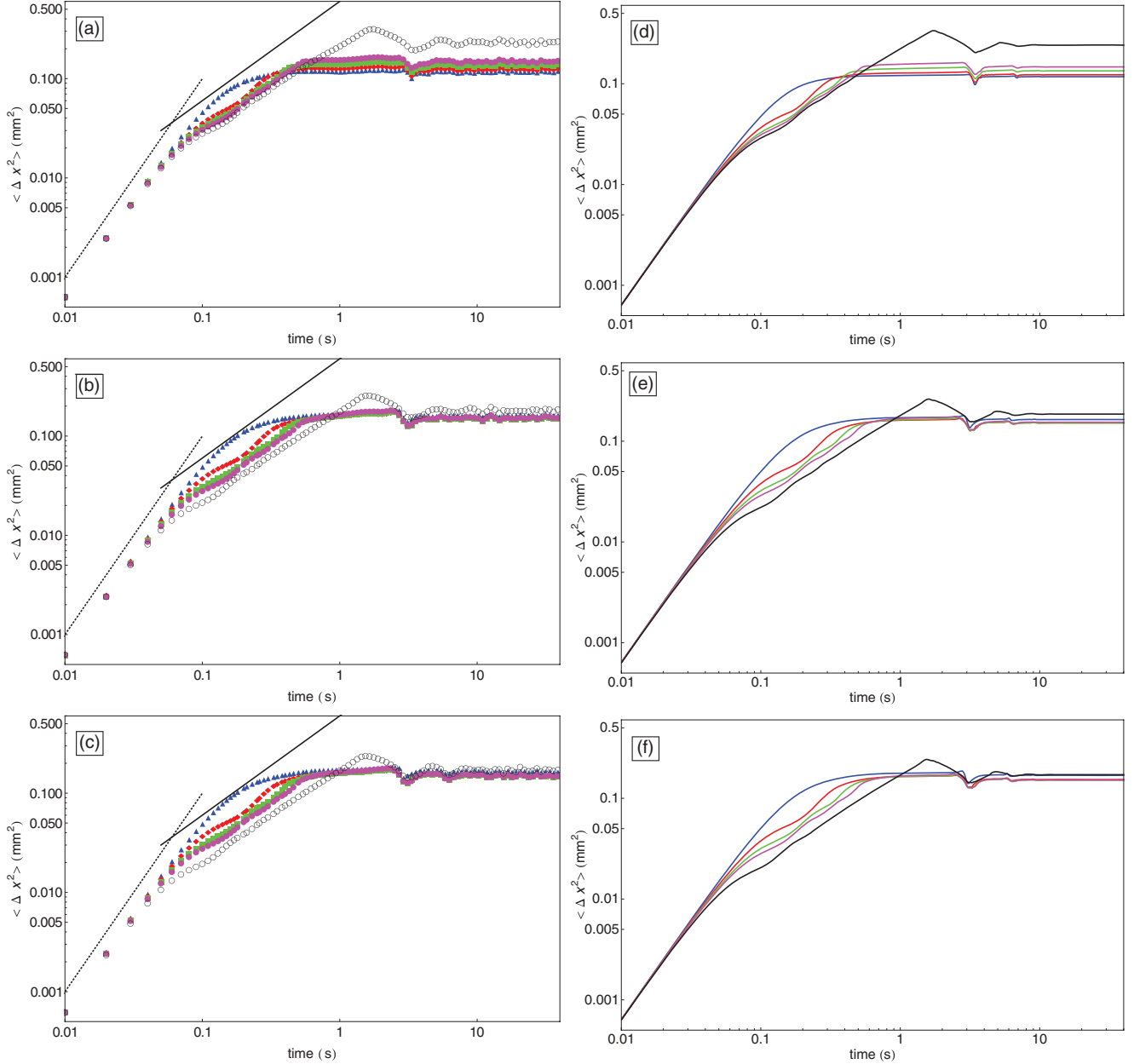
FIG. 3. (Color online) Plot of MSD \langle \Delta u(n,t)^2 \rangle (in \text{mm}^2 ) as a function of time (in s), for a system of 33 particles and a LR confining potential with E_w = 0.1E_0 and \lambda_w = 4 mm [(a) and (d)], \lambda_w = 11 mm [(b) and (e)], and \lambda_w = 30 mm [(c) and (f)]. The damping is \gamma = 1\text{s}^{-1} . We show the particles with n = \pm 16 (blue dots), n = \pm 15 (red squares), n = \pm 14 (green diamonds), n = \pm 13 (magenta triangles down), and n = 0 (black triangles up). Left column: simulations data; right column: calculations. Both axes in Log scales. Dotted lines of slope 2, solid lines of slope 1.
