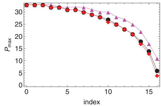
FIG. 15. (Color online) Plot of P_{\max}(n, \lambda_w, E_w) as a function of the particle index n for several LR confining potentials characterized by E_w/E_0 = 0.1 and \lambda_w = 4 mm (magenta triangles), 15 mm (black dots), and 30 mm (red diamonds). The values of P_{\max}(16, 15 \text{ mm}, 0.1E_0) and P_{\max}(16, 15 \text{ mm}, 0.1E_0) may be read in Fig. 11(c)
