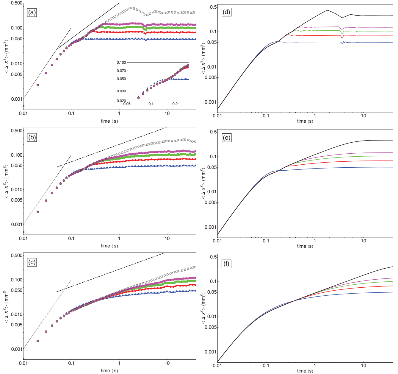
FIG. 2. (Color online) Plot of MSD \langle \Delta u(n, t)^2 \rangle (in \text{mm}^2 ) as a function of time (in s), for a system of 33 particles and for a SW confining potential with \lambda_w = 1 \text{ mm} and E_w = 0.1E_0 . We show the particles with n = \pm 16 (blue dots), n = \pm 15 (red squares), n = \pm 14 (green diamonds), n = \pm 13 (magenta triangles up), and n = 0 (black triangles down). The damping is \gamma = 1 \text{ s}^{-1} [(a) and (d)]; \gamma = 10 \text{ s}^{-1} [(b) and (e)]; \gamma = 60 \text{ s}^{-1} [(c) and (f)]. Left column: simulations data; right column: calculations. Both axes in Log scales. Dotted lines of slope 2, solid lines of slope 1, and dashed lines of slope 1/2. In the inset we zoom on the curves crossing.
