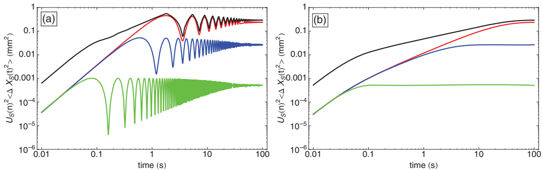
FIG. 13. (Color online) Plot of the variations with time (in s) of the contribution \langle \Delta X_s^2(t) \rangle U_s(0)^2 of the mode s = 1 (red; dark gray, top), s = 3 (blue; medium), s = 33 (green; bottom) to the MSD \langle \Delta u(0, t)^2 \rangle (in \text{mm}^2 ) for a system of 33 particles and a SW confining potential with E_w = 0.1 E_0 and \lambda_w = 1 mm. (a) \gamma = 0.1 \text{ s}^{-1} , (b) \gamma = 60 \text{ s}^{-1} . In black we plot the summation on all modes.
