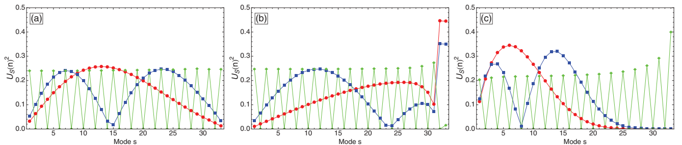
FIG. 11. (Color online) Variations of |U_s(n)| with the mode index s for three different particles, the outermost one ( n = \pm 16 ) (red dots), the next one ( n = \pm 15 ) (blue squares), and the central particle ( n = 0 ) (green diamonds). (a) SW confining potential with \lambda_w = 1 mm, E_w/E_0 = 0.1 ; (b) HW confining potential with \lambda_w = 0.48 mm, E_w/E_0 = 0.005 ; (c) \lambda_w = 15 mm, E_w/E_0 = 0.1 .
