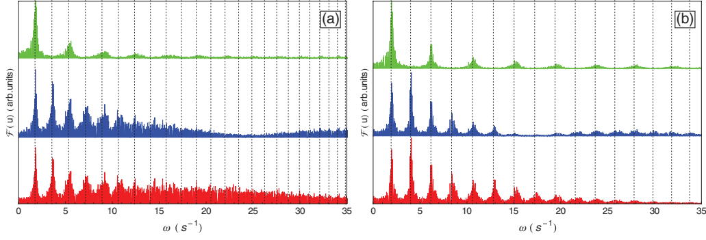
FIG. 12. (Color online) Plot of the power spectra (arb. units) of the particles trajectories as a function of the frequency \omega ( \text{s}^{-1} ) for particles n = \pm 16 (bottom), n = \pm 15 (center) and n = 0 (top). (a) SW confinement: \lambda_w = 1 mm, E_w/E_0 = 0.1 . (b) LR confinement: \lambda_w = 15 mm, E_w/E_0 = 0.1 . The dotted lines indicate the first 24 (a) and 16 (b) calculated frequencies.
