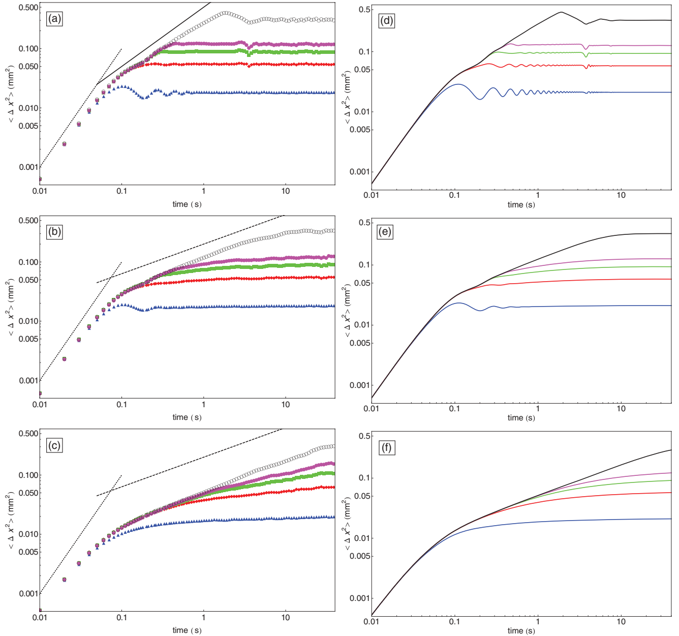
FIG. 1. (Color online) Plot of MSD \langle \Delta u(n,t)^2 \rangle (in \text{mm}^2 ) as a function of time (in s), for a system of 33 particles and HW confinement with \lambda_w = 0.48 mm and E_w = 0.0095 E_0 . We show the particles with n = \pm 16 (blue dots), n = \pm 15 (red squares), n = \pm 14 (green diamonds), n = \pm 13 (magenta triangles up), and n = 0 (black triangles down): \gamma = 1 \text{ s}^{-1} [(a) and (d)]; \gamma = 10 \text{ s}^{-1} [(b) and (e)]; \gamma = 60 \text{ s}^{-1} [(c) and (f)]. Left column: simulations data; right column: calculations. Both axes in Log scales. Dotted lines of slope 2, solid lines of slope 1, and dashed lines of slope 1/2.
