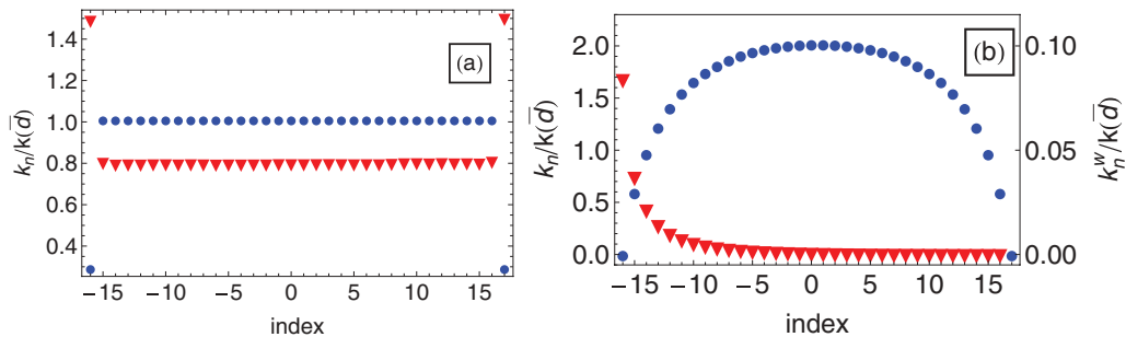
FIG. 9. (Color online) Dimensionless stiffness as a function of the particle index, for 33 particles. (a) SR confinement. Interparticle stiffness k_n/k(\bar{d}) for a SW (blue dots) and HW (red triangles). (b) LR confinement, \lambda_w = 11 mm, E_w = 0.1 E_0 . Interparticle stiffness k_n/k(\bar{d}) (left axis, blue dots) and confinement stiffness -\frac{\partial F_w}{\partial x}(L/2 + x_n^*)/k(\bar{d}) (right axis, red triangles).
