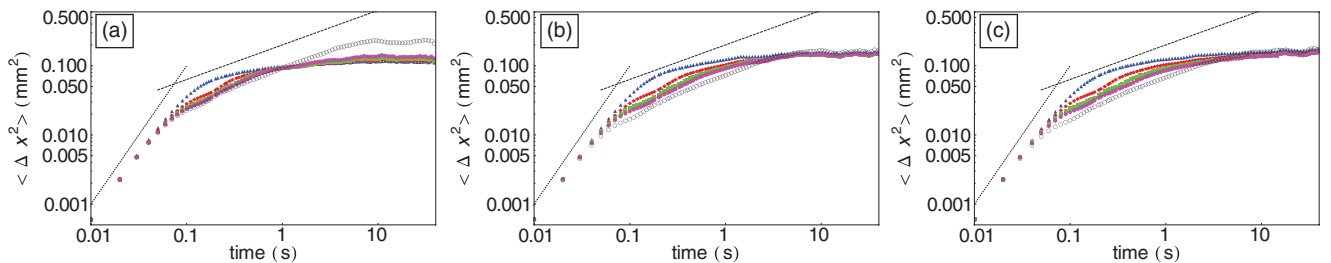
FIG. 5. (Color online) Plot of MSD \langle \Delta u(n, t)^2 \rangle (in \text{mm}^2 ) as a function of time (in s), for a system of 33 particles and a LR confining potential with E_w = 0.1E_0 and \lambda_w = 4 \text{ mm} (a); 11 mm (b), 30 mm (c). The damping is \gamma = 10 \text{ s}^{-1} . We display the particles with n = \pm 16 (blue dots), n = \pm 15 (red squares), n = \pm 14 (green diamonds), n = \pm 13 (magenta triangles up), and n = 0 (black triangles down). Dotted lines of slope 2, and dashed lines of slope 1/2
