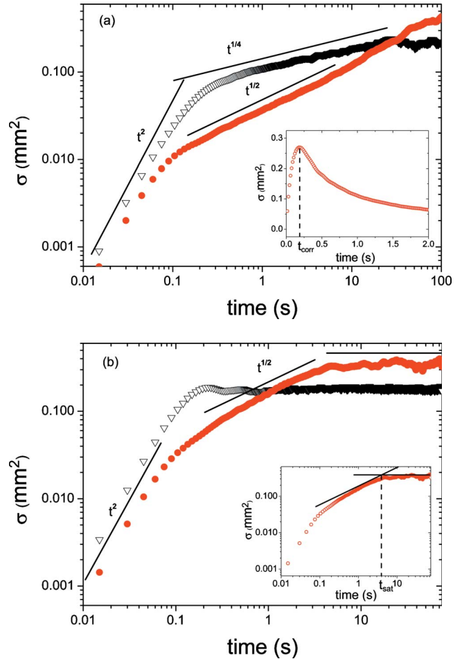
FIG. 6. (Color online) Plot of the m.s.d. (in \text{mm}^2 ) of the central (filled disks) and the outermost balls (empty triangles) as a function of time (in s.) for V = 1000\text{ V} (a) and 1300\text{ V} (b). Three different regimes can be observed. Their extensions vary according to the ball position and the applied voltage. Notice the “curve crossing” which is characteristic of the diffusion in finite channel and indicates different dynamic regimes according to the ball position. The insert in 6a and 6b, respectively, explain the measurements of t_{\text{corr}} and t_{\text{sat}} .
