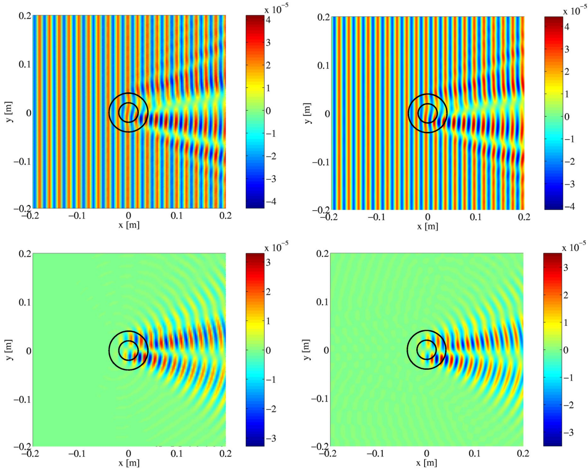
FIG. 6. Sound field resulting from the interaction of an incident plane monochromatic sound wave (propagating from the left to the right of the domain, \lambda/L^*=1 ) with the mean flow U_2 [Eq. (50)], \mathcal{M}\approx 0.1 , \beta\approx 12 . Left-upper, sound wave \rho_s from the partial-wave computations; right-upper, sound wave \rho_s from the direct numerical simulation. Left-lower, scattered sound wave \rho_{scat} from the partial-wave computations; right-lower, scattered sound wave \rho_{scat} from the direct numerical simulation. Circles locate the position of the two opposite sign vorticity domains. Units are in meters on each axis.
