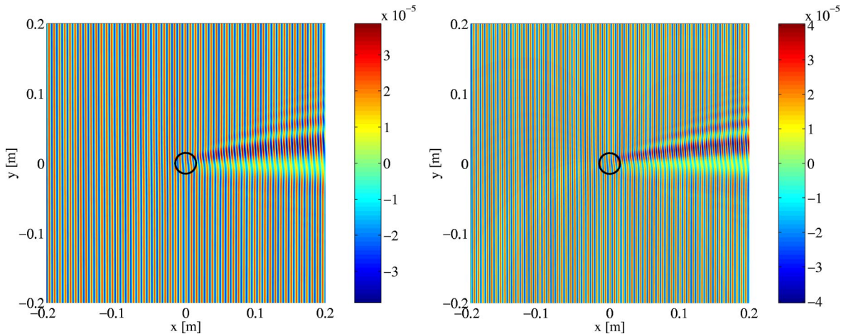
FIG. 9. Sound wave \rho_s resulting from the interaction of an incident plane monochromatic sound wave (propagating from the left to the right of the domain) with the mean flow U_3 [Eq. (77)], \mathcal{M}\approx 0.039 . Partial-wave computations with left, \lambda/L^*=3/4 , \beta\approx 13.1 ; right, \lambda/L^*=0.625 , \beta\approx 15.8 . Circle locates the position of the vortex core (rotating counterclockwise). Units are in meters on each axis.
