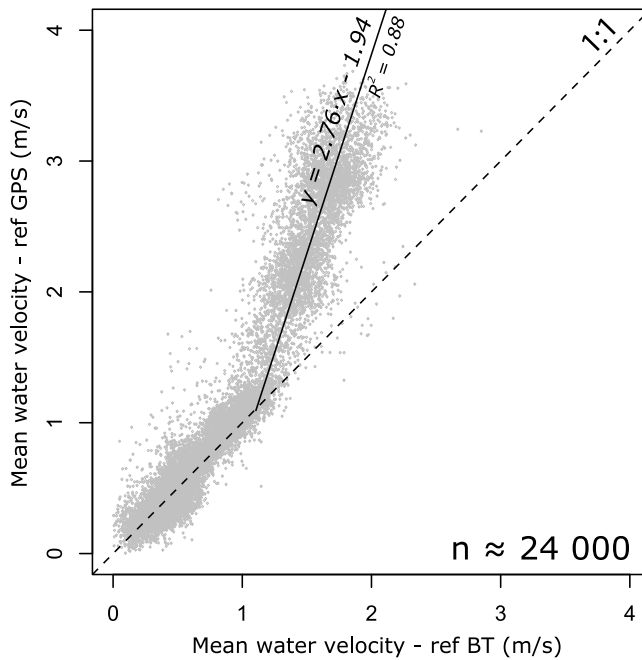
Figure 3. Water column mean velocity as measured simultaneously from bottom tracking mode (BT) of the ADCP (assuming fixed river bottom) and from GPS mode (GPS position as reference). These two modes yield similar results up to \sim 1.1 m/s but diverge for higher water velocities. For higher water velocities significant bed motion is detected. This result can be used to correct measurements where GPS data are not available and that would otherwise be biased toward significantly lower water velocities. These data were generated from \sim 24000 vertical velocity profiles (ensembles) acquired on the Ganga in 2008 and 2010.
