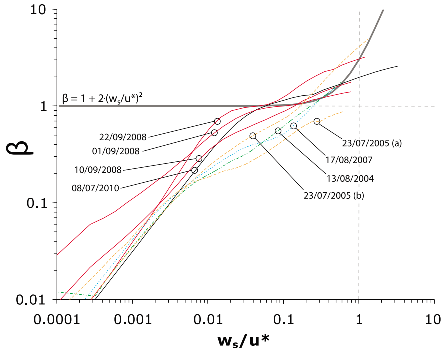
Figure 9. Evolution of \beta as function of w_s/u^* for the different profiles of the Ganga at Harding Bridge. The relation derived by van Rijn [1984b], \beta = 1 + 2(w_s/u^*)^2 , is also plotted for comparison.
