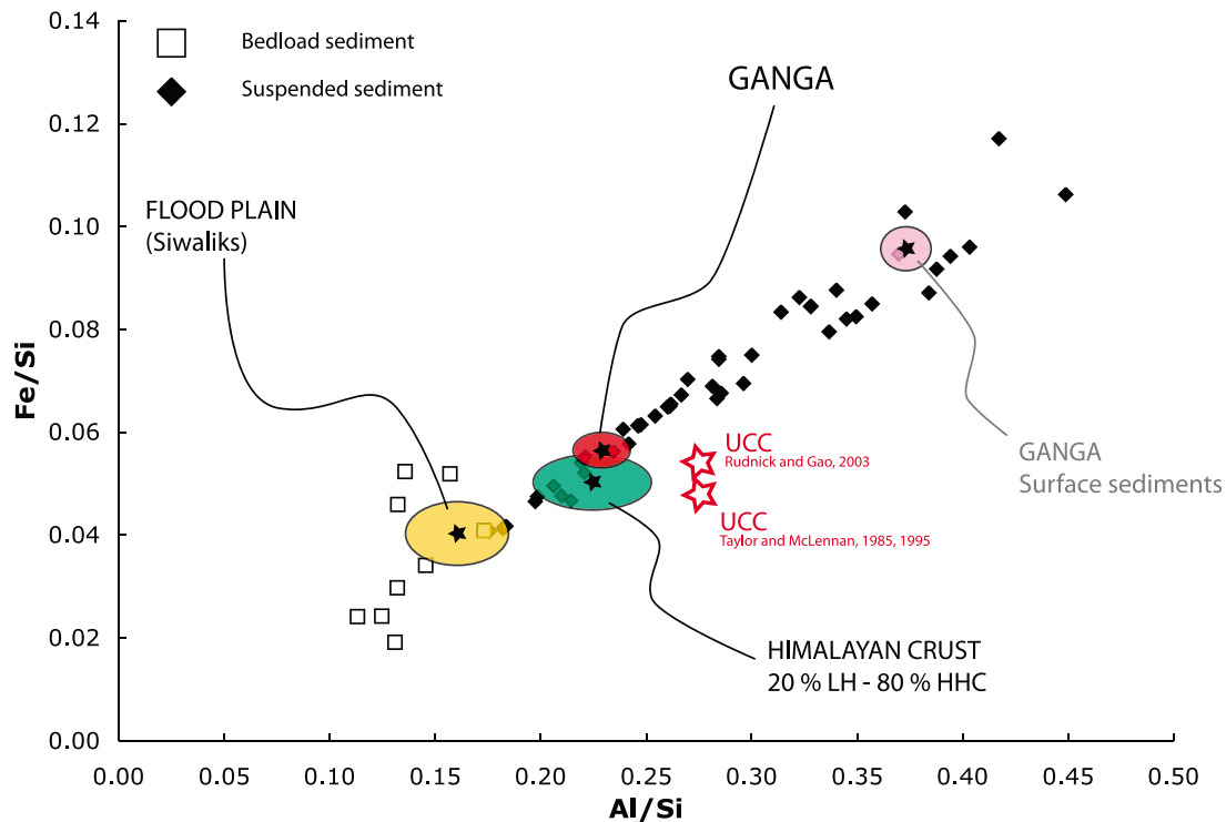
Figure 15. Al/Si versus Fe/Si for the Ganga sediments as modeled in this work, Siwaliks as modern flood-plain sediments analogs, Himalayan crust from Galy and France-Lanord [2001] and Ganga surface sediments for comparison (molar ratios). Individual sampled suspended sediments and dredged bed load samples are plotted as black diamonds and open squares respectively. Also plotted is the Upper Continental Crust (UCC) as defined by Taylor and McLennan [1985, 1995] and Rudnick and Gao [2003].
