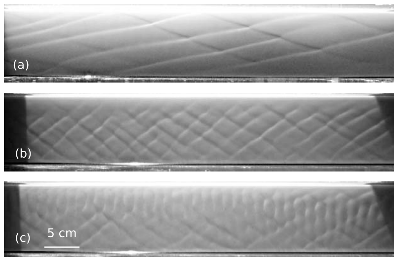
Figure 7. Various bed forms observed in our experiment (flow is from right to left). (a) Large rhomboid pattern ( F = 1.76 , S = 0.03 , and \theta = 0.616 ). (b) Small rhomboid pattern ( F = 0.95 , S = 0.015 , and \theta = 0.485 ). (c) Rhomboid pattern mixed with ripples ( F = 1.01 , S = 0.015 , and \theta = 0.504 ).
