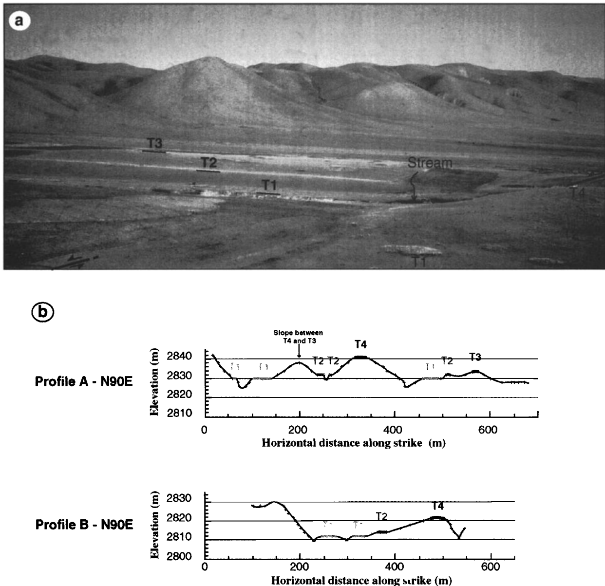
Figure 3. (a) Northeast looking view of site 1. Flat, gently south sloping terrace ledges T1, T2, and T3 are clear in middle ground, on left bank of offset stream channel. T4 is visible south of fault to the right. (b) E-W profiles, A and B, derived from vertical sections of DEM, north and south of fault, respectively (location on Plates 2b and 2c). Crosses are intersections of profile lines with contour lines of DEM. Vertical exaggeration is 4. Four different terrace levels are identified (see text).
