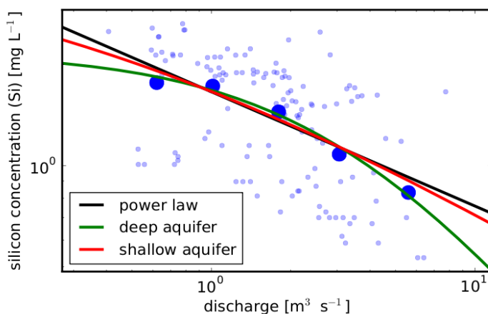
Figure 5 Concentration of Silicon as a function of discharge in the Ürümqi River, China (small blue dots). All three models have two adjustable parameters. Power-law: c = 1.7Q^{-0.34} (if c and Q are expressed in \text{mgL}^{-1} and \text{m}^3 \text{ s}^{-1} respectively); deep aquifer: c_s = 2.2 \text{ mgL}^{-1} and Q_c = 3.3 \text{ m}^3 \text{ s}^{-1} ; shallow aquifer: c_s = 5.1 \text{ mgL}^{-1} and Q_c = 0.45 \text{ m}^3 \text{ s}^{-1} . The large blue dots represent bin averaged data
