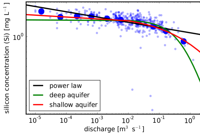
Figure 6 Concentration of Silicon as a function of discharge in a stream of the Mont Lozère, France (small blue dots). All three models have two adjustable parameters. Power-law: c=1.1Q^{-0.05} (if c and Q are expressed in \text{mgL}^{-1} and \text{m}^3\text{s}^{-1} respectively); deep aquifer: c_s=1.5\text{ mgL}^{-1} and Q_c=0.65\text{ m}^3\text{s}^{-1} ; shallow aquifer: c_s=1.7\text{ mgL}^{-1} and Q_c=2.2\text{ m}^3\text{s}^{-1} . The large blue dots represent bin averaged data
