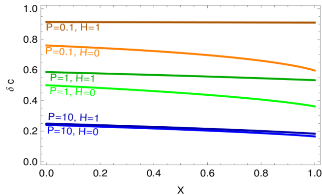
Figure 2 Distribution of the non-dimensional solute concentration along an aquifer, for various values of the parameters defined in relation (9). The water divide is at X=0 , whereas X=1 corresponds to the aquifer outlet into the river
