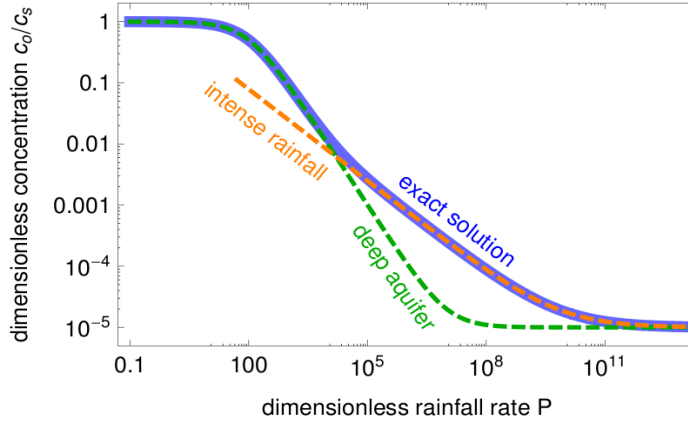
Figure 3 Theoretical concentration-discharge relationships for H=100 and c_r/c_s=10^{-5} . The complete solution requires the numerical integration of equation (8), whereas the two asymptotic behaviors correspond to the analytic expressions (13) and (20)
