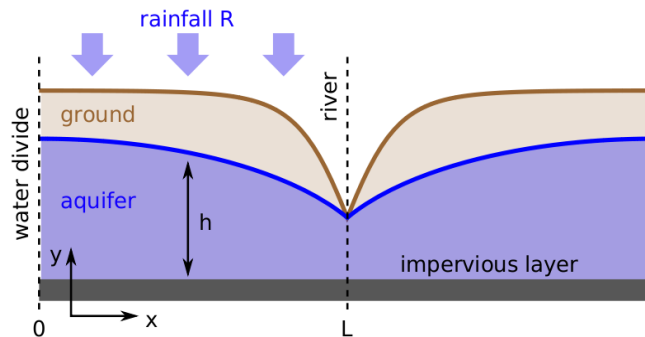
Figure 1 Schematics of an aquifer, and associated notations. The rainfall water fills the aquifer, which in turns flows into a stream. The porous rock is dissolved by groundwater, the concentration of which depends on the shape h(x) of the aquifer
