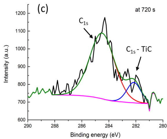
Figure 3: a) Atomic percentages (%) -versus- Etching time (s) for a Si/SiO 2 /PPF/BTB 9 /Ti 2 /Au 20 b) Titanium high resolution XPS signal, c) Carbon high resolution XPS signal.
