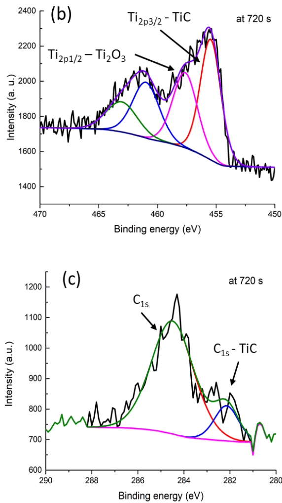
Figure 3: a) Atomic percentages (%) -versus- Etching time (s) for \text{a-Si/SiO}_2/\text{PPF/BTB}_9/\text{Ti}_2/\text{Au}_{20} b) Titanium high resolution XPS signal, c) Carbon high resolution XPS signal.
