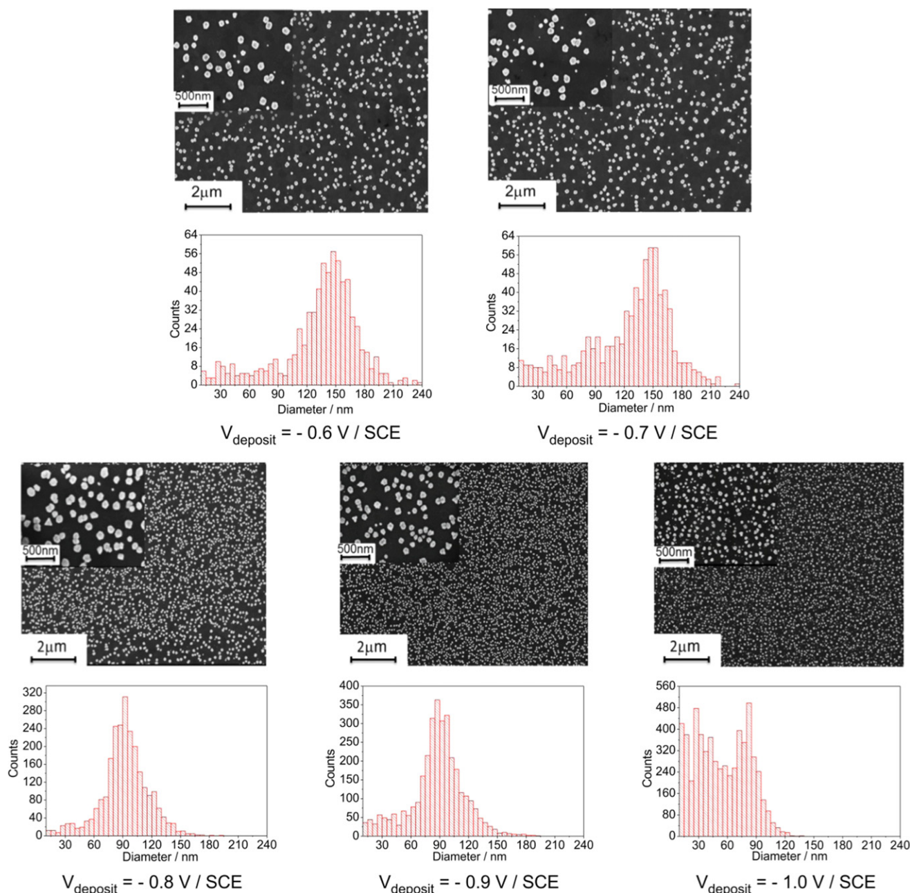
Figure 2. SEM images of AuNPs electrodeposited onto ITO at various reduction potentials ( -0.6 to -1.0 V/SCE and fixed total charge density ( Q = 20 mC cm ^{-2} ), and corresponding AuNP diameter distribution histograms.
