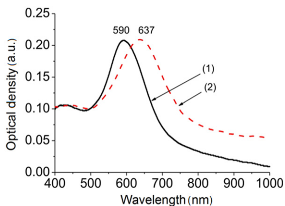
Figure 4. Optical extinction spectra of an AuNP electrode obtained by electrodeposition ( -0.8 V/SCE and 20 \text{ mC cm}^{-2} ), before (curve 1) and after (curve 2) BTB deposition.
