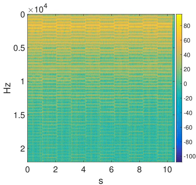
Fig. 9: Spectrogram of a priority car alarm signal
