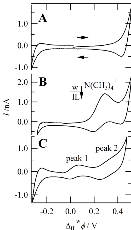
Figure 1: Cyclic voltammograms obtained at a w|P 888 B(C 6 F 5 ) 4 , 25 \mu m diameter, micro-interface housed at the tip of a pulled capillary using (A) Cell 1, without CMPO added, (B) Cell 2, and (C) Cell 1 with y = 60 mM of CMPO added to the IL phase. All traces were obtained at a scan rate of 0.020 V s -1 and with a heating mantle at 60 °C.
