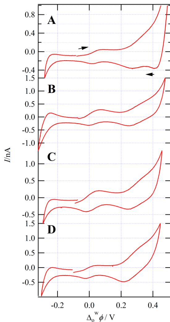
Figure 2: Cyclic voltammograms recorded using Cell 1 with the concentration of CMPO (y) varied in the IL phase from 30 to 85 mM from A to D. All other instrument parameters were the same as detailed in Figure 1.
