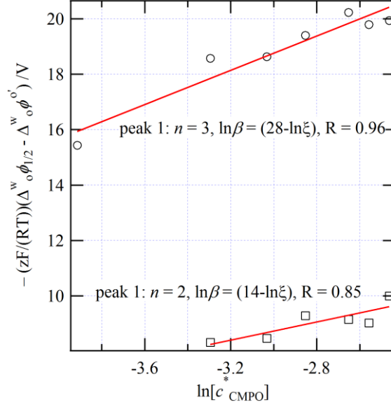
Figure 3: Trend of -zF/(RT)(\Delta_{IL}^w\phi_{ML_n^z,1/2} - \Delta_{IL}^w\phi^{o'}) versus \ln[c_{CMPO}] obtained from the shift in \Delta_{IL}^w\phi_{ML_n^z,1/2} (see Figure 2). Red traces indicate the linear curve fitting applied to the data with metal:ligand (1: n ) stoichiometry, overall complexation constant \beta ( \xi = \sqrt{D_{IL}/D_w} ), and Pearson's R values indicated.
