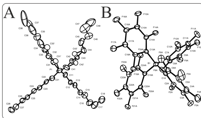
Figure 5: Structure of P_{888}B(C_6F_5)_4 ( C_{56}H_{68}BF_{20}P ) as determined by X-ray diffraction. (A) Oak Ridge Thermal Ellipsoid Plot (ORTEP) of P_{888}^+ showing naming and numbering scheme. Ellipsoids are at the 50% probability level and hydrogen atoms were omitted for clarity. The disordered portion of the cation is depicted as “open” ellipsoids and bonds. (B) ORTEP of B(C_6F_5)_4^- showing naming and numbering scheme. Ellipsoids are at the 25% probability level for clarity.
