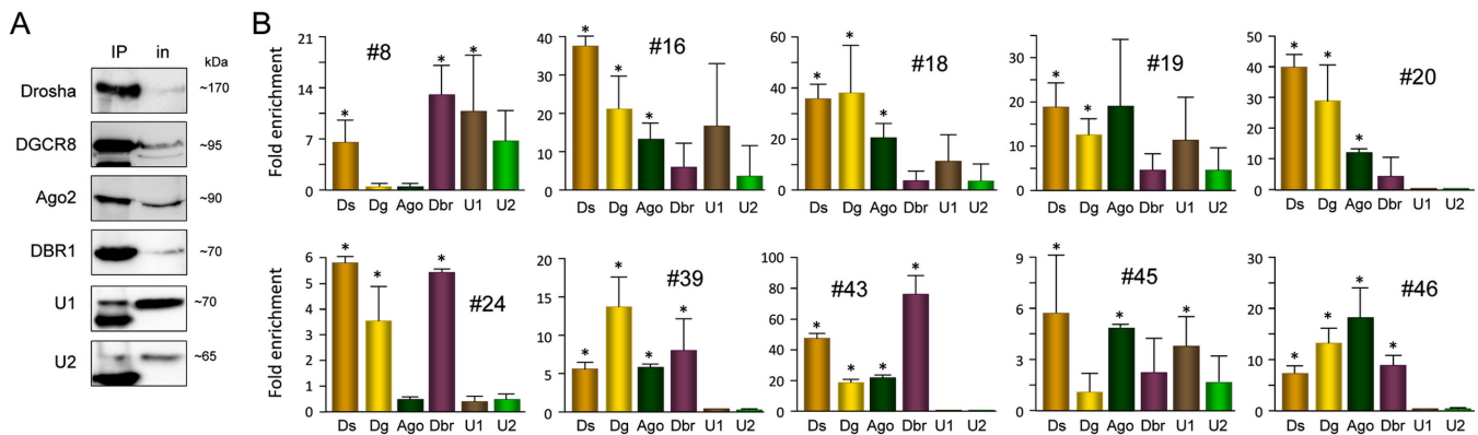
Figure 5. SID interactions with miRNA pathway key factors. (A) Native RIP was performed using the indicated antibodies and the effective protein precipitation was confirmed by western blotting. IP, immunoprecipitation; in, 5% input. (B) Co-precipitated RNAs were extracted as described in Material and Methods section ( n = 2 ). Quantitative PCR were performed using specific primer pairs (Supplementary Table S2) to amplify SID #8, #16, #18, #19, #20, #24, #39, #43, #45 and #46. Amount of immunoprecipitated material is expressed as fold enrichment compared to irrelevant antibody. Ds, Drossha; Dg, DGCR8; Ago, Ago2; Dbr, DBR1; U1, snRNP70; U2, U2AF65. Significant differences with irrelevant antibody were assessed using Student's t -test ( *P < 0.05 ). Error bars represent standard error at the mean (SEM).
