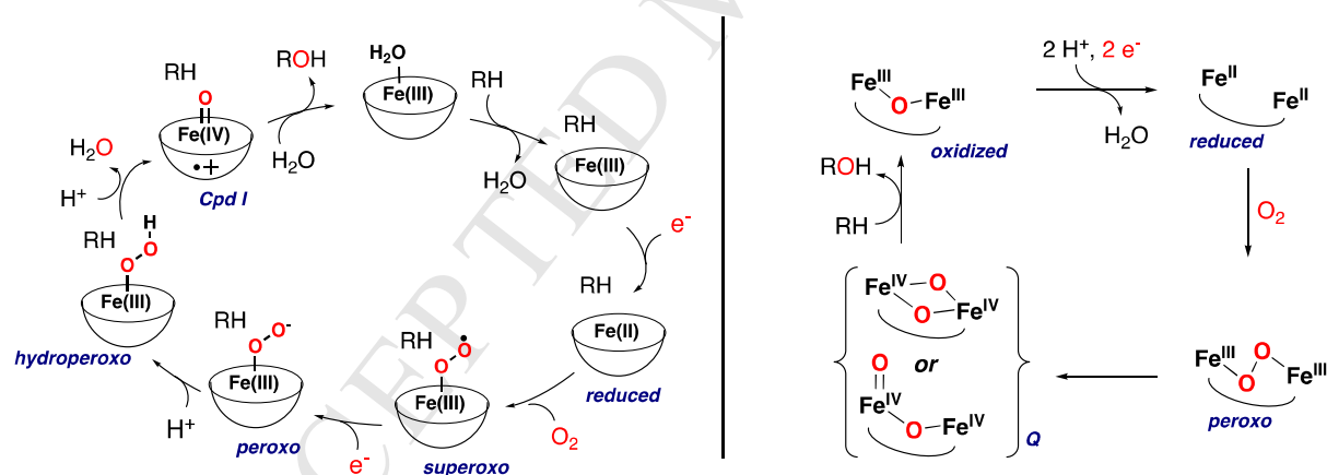
Figure 1. Left and right panels describe the catalytic cycles of P450 and sMMO, respectively (RH designates a substrate). The comparison between the two mechanisms evidences that the electrons are consumed in two different steps in P450, whereas there is only one reductive step in sMMO.
