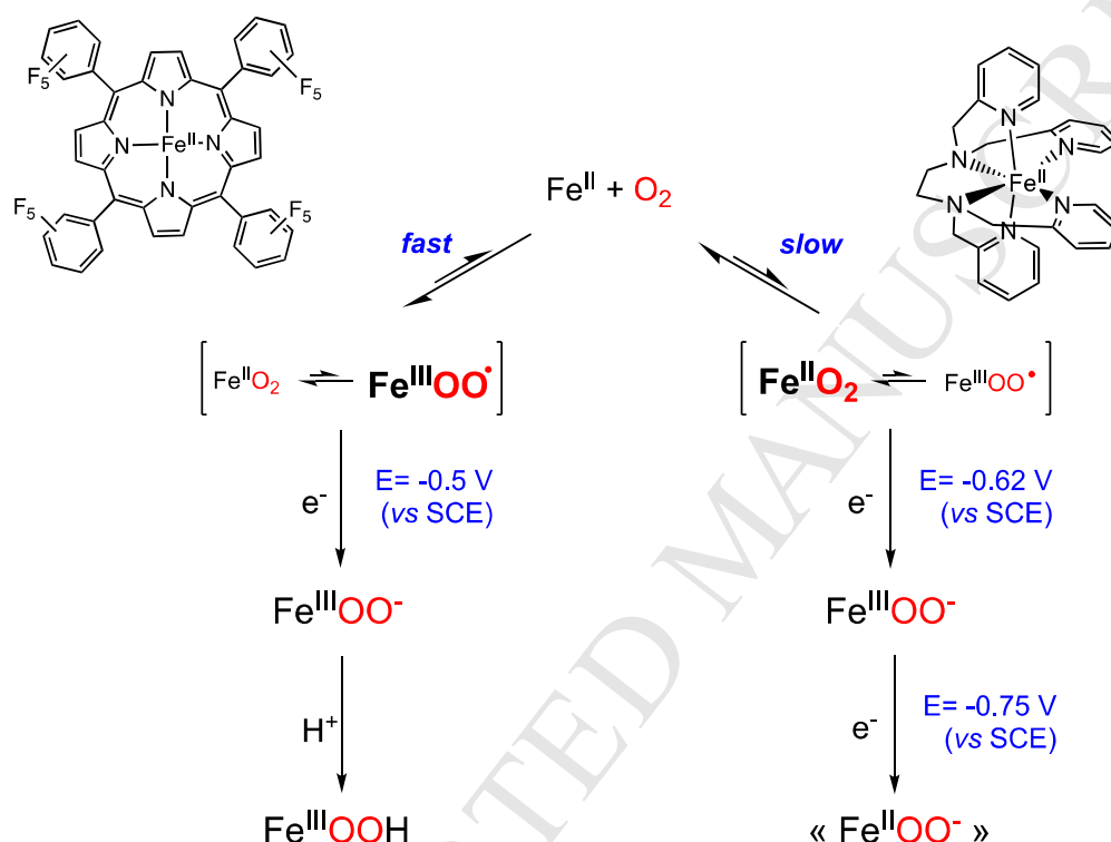
Figure 4: Electrochemical reductive activation of \text{O}_2 by a porphyrinic (left panel) or non porphyrinic (right panel) iron complex underlining basic differences between the two classes of complexes. Adapted from references [34] and [35], respectively.
