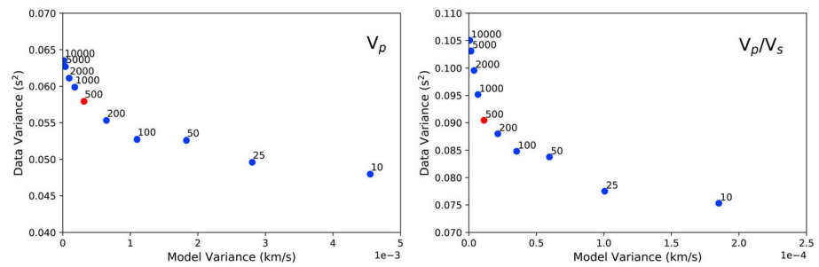
Figure 3. Trade-off curves for the reduction of data variance versus increase in model variance. Blue circles represent the values after one iteration of the inversion for different damping values, ranging from 10 to 10,000. The red circles represent the optimum damping values for both the V_p and V_p/V_s models, which were used in the final inversion.
