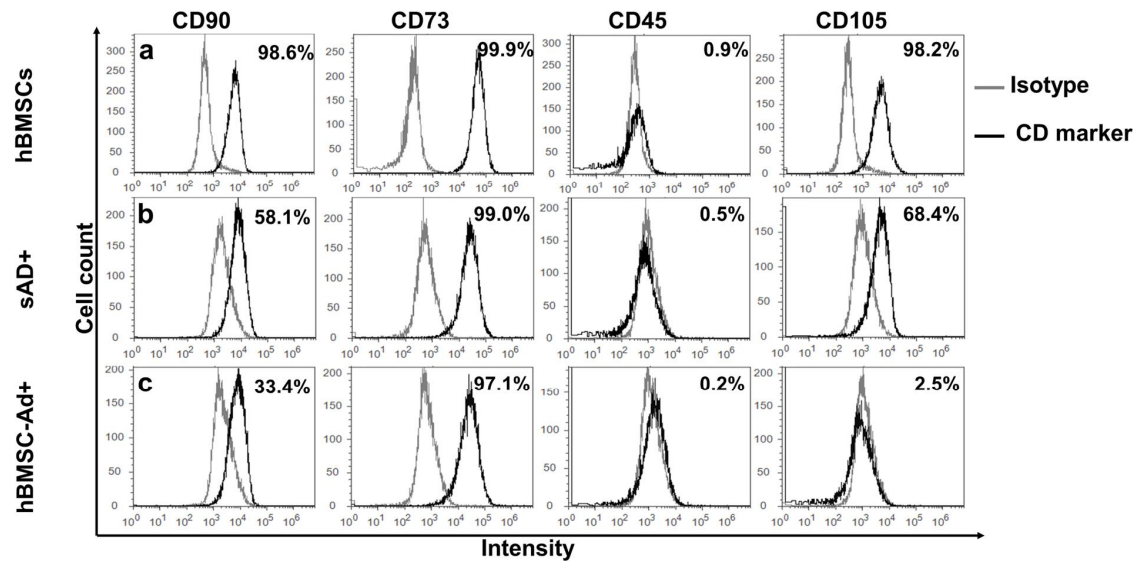
Figure S1: Phenotypic characterization regarding surface markers CD90, CD73, CD45 and CD105 for hBMSC, sAD+ and hBMSC-Ad+ cell populations: Mouse antibodies directed against each human surface marker (all purchased from Miltenyi Biotec) were used according to manufacturer's instructions. 500,000 cells were washed with PBS, trypsinized, and centrifuged at 1,500 rpm for 5 min. Each supernatant was discarded and the respective cell pellet was re-suspended in PBS-EDTA (2 mM)-BSA (0.5%), separated in two equal fractions, and centrifuged again at 1,500 rpm. These cells were incubated 15 min in the presence either of CD90-FITC, of CD73-PE, of CD105-vioblu, of CD45-PerCP, or of isotype matched-controls of each marker tested. After centrifugation, the cells were re-suspended before analysis using flow cytometry. The black histograms represent CD-labeled cell populations and the gray ones represent isotype-labeled cell populations. These results are expressed as percentage of the marker positive labeled-cells compared to the respective isotype labeled cells.
