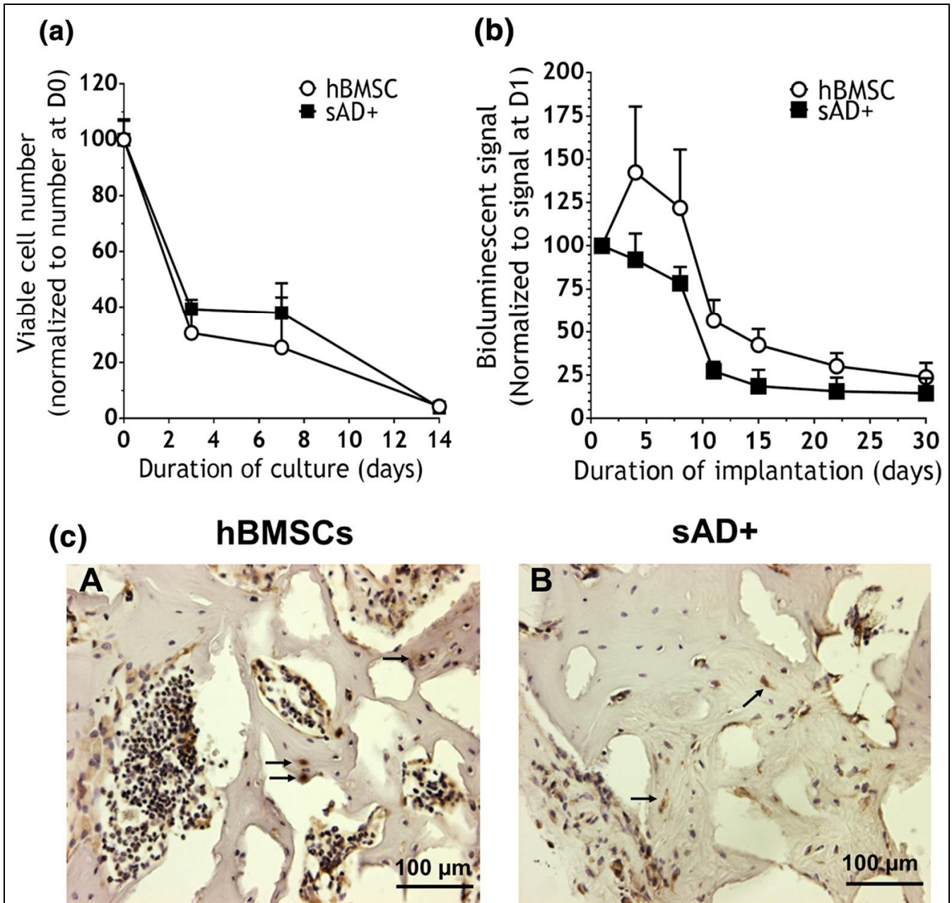
Figure 4: Fate of the sAD+ and hBMSC cells under ischaemic conditions in vitro and in vivo. (a) Time-course of the cell viability of both hBMSCs and sAD+ cells cultured under (near-anoxia, glucose depletion, and serum depletion) ischaemic conditions. The cell viability was assessed after Hoescht 33442-staining (total nuclei) and propidium iodide-staining (dead cells) followed by flow cytometry cells analysis. The values are means \pm SEM. (n = 6). Two-ways ANOVA, p > .05 . (b) In vivo cell viability of both hBMSCs(Luc) and sAD+(Luc) cells determined by bioluminescent imaging after ectopic implantation in nude mice for 30 days. The photon fluxes were normalized to those obtained at Day 1 post-implantation. The values are means \pm SEM. (n = 6). Two-way ANOVA, p > .05 (c) Implanted hBMSC (frame cA) or sAD+ cells (frame cB), still present in the constructs explanted 8 weeks post-implantation were detected on paraffin-treated sections following immunostaining against human \beta -2-microglobulin. The black arrows points at positive labelled osteocytes. hBMSCs = human adult multipotent bone marrow stromal cells
