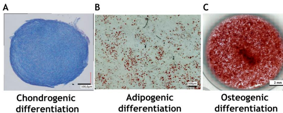
Figure S2: Multilineage potential of hBMSCs. (A): For the chondrogenic differentiation 2,5x10 4 hBMSC cells were cultured in micromass pellets in the presence of high-glucose DMEM medium containing 50 µg/ml ascorbic acid-2 phosphate, 100 nM dexamethasone, 1% (v/v) ITS and 10 ng/ml TGFβ3 for 21 days (Mackay et al. Tissue eng, 1998). At that time, the hBMSCs cell aggregates were fixed, embedded in paraffin and processed for histochemical analysis; tissue section was stained with Alcian Blue, to detect sulfated proteoglycans (scale 100 µm). (B) For adipogenic and (C) osteogenic differentiation potentials, hMSCs were cultured either in an adipogenic (AD) medium for 21 days and stained with oil red O solution (scale 500 µm) or in an osteogenic (OS) medium for 28 days and stained with alizarin red (scale 2000 µm) as described in the Materials and Methods section.
