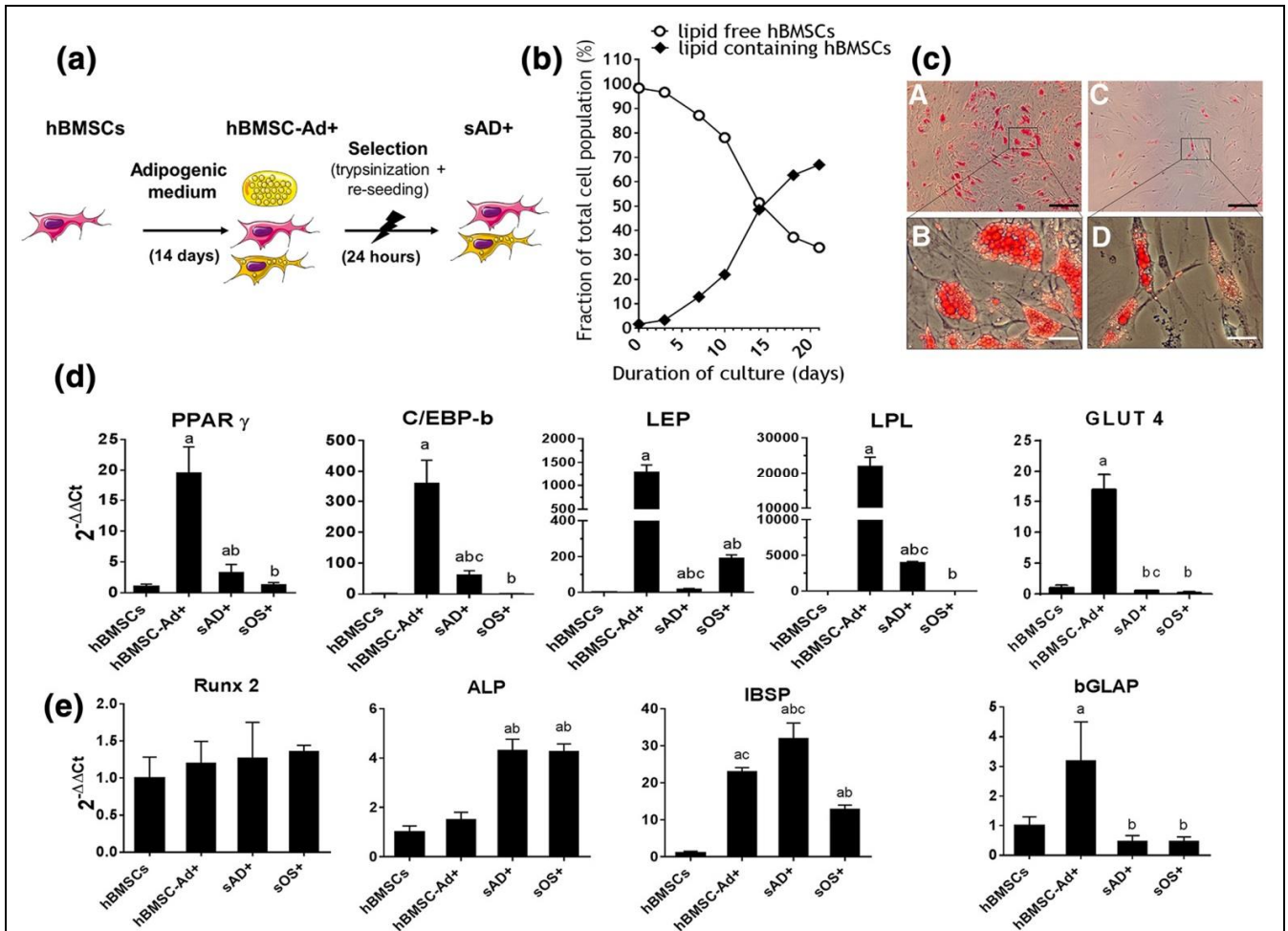
Figure 1: Characterization of the sAD + cell population. (a) Experimental design for hBMSC predifferentiation: hBMSCs were cultured in adipogenic medium for 14 days followed by a trypsinizing and reseed-based selective-step that eliminated mature adipocytes, resulting in a select, heterogeneous, adipogenic predifferentiated sAD + cell population. (b) Time-course of the lipid-containing hBMSC population assessed by flow cytometry during hBMSC adipogenic differentiation for 21 days. (c) Representative images of Oil Red O staining of hBMSC-Ad + cells (prior to the selective step; cA and cB) and sAD + cells (24 hr after the selective step; cC and cD); black scale bar = 200 \mu m, white scale bar = 60 \mu m. (d, e) Gene expression of hBMSCs, BMSC-Ad + cells, sAD + cells, and sOS + cells (both 24 hr after the selective step), pertinent to adipogenesis and osteogenesis. (d) Results from RT-qPCR analysis of the adipogenesis-related gene expression: Peroxisome proliferator-activated receptor gamma (PPAR \gamma ), CCAAT-enhancer-binding proteins (C/EBP- \beta ), leptin (LEP), lipoprotein lipase (LPL), and glucose transporter type 4 (GLUT4). (e) Results from RT-qPCR analysis of the osteogenesis-related gene expression: Alkaline phosphatase (ALP); runt-related transcription factor 2 (RUNX2), integrin binding sialoprotein (IBSP) and bone gamma-carboxyglutamate (Gla) protein (bGLAP). Gene expressions were normalized first to that of the respective 18S (internal standard), and then to results obtained for hBMSCs (2 -ΔΔCt ) format. Values are means \pm SEM from three separate experiments. One-way ANOVA with Tukey's post-hoc test. (a) p < .05 versus hBMSCs. (b) p < .05 versus hBMSC-Ad + cells. (c) p < .05 versus sOS + cells. hBMSCs = human adult multipotent bone marrow stromal cells.
