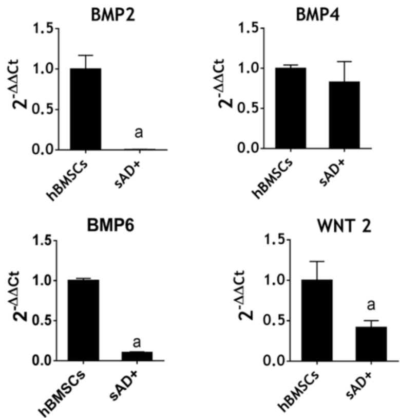
Figure S6: BMPs and Wnt Gene expression of hBMSCs and sAD+ cells. Results from RT-qPCR analysis of the following genes: Bone morphogenetic 2 (BMP2), Bone morphogenetic 4 (BMP4), Bone morphogenetic 6 (BMP6) and Wingless-type MMTV integration site 2 (Wnt2). The gene expression was normalized first to that of the respective 18S (internal standard), and then to results obtained with undifferentiated hBMSCs ( 2^{-\Delta\Delta Ct} ) format). Values are means \pm SEM. (n = 3). These data were analyzed using Mann-Whitney test. (a) p < 0.05 vs. hBMSCs.
