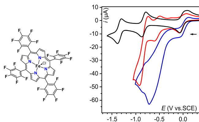
Figure 1. (left) Molecular structure of Fe III (F 20 TPP)Cl. (right) CVs at a glassy-carbon-disk electrode of a 1 mM solution of 1 in DMF + TBAPF 6 (0.1 M), with \nu = 0.1 \text{ V s}^{-1} and T = 293 \text{ K} : under argon (black trace); under O 2 (air saturated, 1 mM) (red trace); under O 2 with 10 mM HClO 4 (blue trace).
