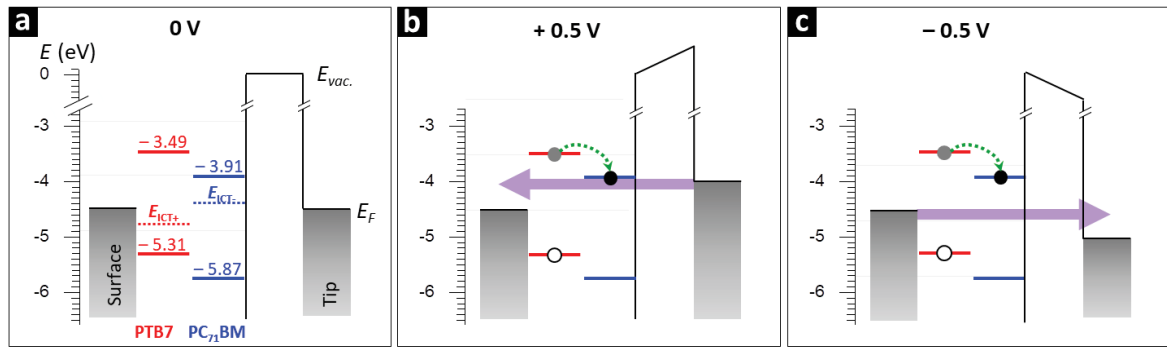
26 27 28 29 30 31 32 33 34 35 36 37 38 39 Figure 8: Energetic diagrams of the metal-PTB7-PC 71 BM//metal junction. (a) Thermodynamic equilibrium situation. Charge transfer between gold and polaronic levels E_{ICT+} and E_{ICT-} of the polymer is found to be unfavored[46]. (b) Non-equilibrium situation under a bias voltage of V_t = +0.5 V. (c) Non-equilibrium situation under a bias voltage of V_t = -0.5 V.
