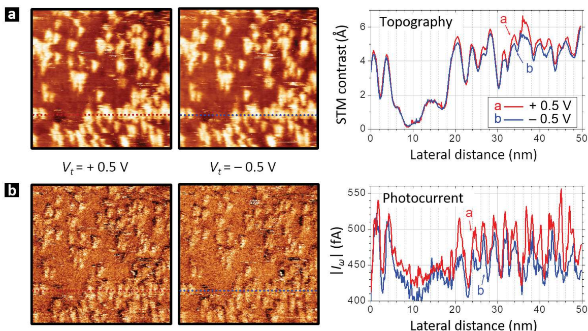
Figure 6: LA-STM images and profiles of the PTB7/PC 71 BM layer on Au(111) obtained by a double sweep of each scan line at V_t = +0.5 \text{ V} and V_t = -0.5 \text{ V} respectively. (a) Topography at I_t = 10 \text{ pA} . (b) Modulated photocurrent map I_\omega at \mathcal{P}_o = 75 \text{ mW} and f_L = 20 \text{ kHz} . The thermal drift of the STM under light irradiation is clearly visible, due to a relative long data acquisition time ( ca. 20 mn per couple of images).
