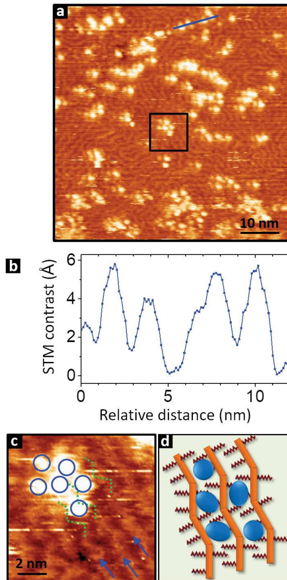
Figure 3: (a) STM image ( 60 \times 60 \text{ nm}^2 ; V_t = +0.6 \text{ V} ; I_t = 50 \text{ pA} ) showing the PC 71 BM islands drop casted on PTB7/Au(111). (b) Cross section extracted from image (a). (c) Magnified image of PTB7/PC 71 BM junctions highlighting the preferential adsorption sites of PC 71 BM on PTB7 (template effect). (d) Sketch of the D/A system.
