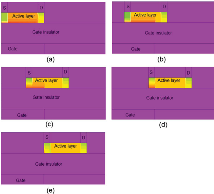
Figure 4. Hole concentration distribution in organic TFTs for gate voltage = drain voltage = -40 V; color-coded hole concentration values; represented by a continuous distribution from a maximum of 10^{19} to a minimum of 0 from red to purple, respectively. L_M is varied (a) 0 \mu\text{m} , (b) 20 \mu\text{m} , (c) 40 \mu\text{m} , (d) 60 \mu\text{m} , and (e) 70 \mu\text{m} .
