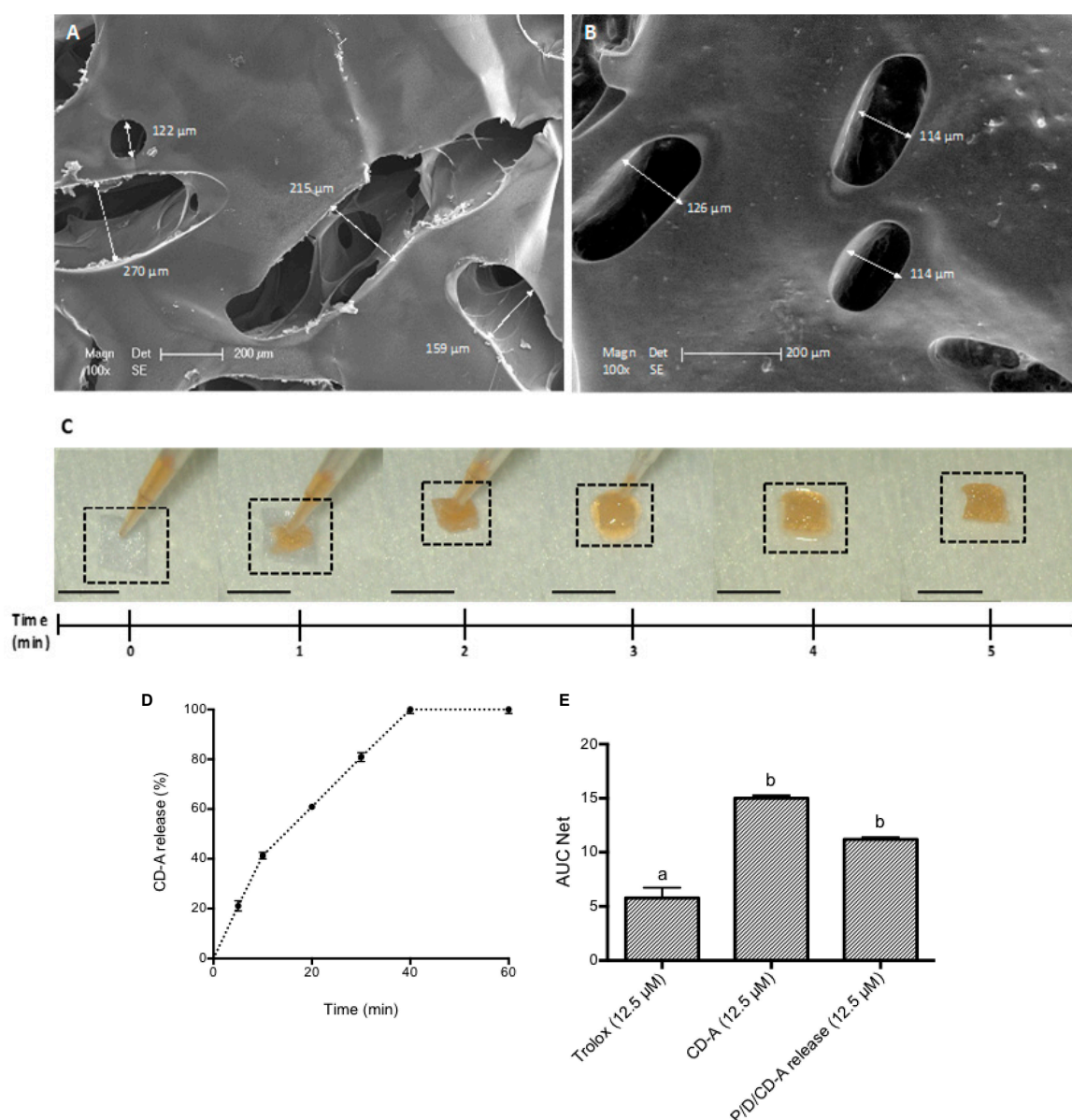
Figure 1. Environmental scanning electron microscopy (ESEM) of the (A) pullulan/dextran (P/D) scaffold and (B) P/D/hydroxypropyl- \beta -cyclodextrin-astaxanthin (CD-A) scaffold. (C) P/D scaffolds were loaded with 10 \mu\text{L} of either saline solution or CD-A until complete absorption. (D) CD-A release kinetics from the P/D scaffolds during 60 min in PBS (pH 7.4). The results indicate mean \pm SD ( n = 46 ). (E) Antioxidant activity evaluation of CD-A and P/D/CD-A release product at 12.5 \mu\text{M} compared to Trolox at 12.5 \mu\text{M} standard antioxidant; results are presented as area under the curve (AUC) net values; the results are expressed as mean \pm SD ( n = 46 ); values connected with the same letter (a, b) are not significantly different considering p < 0.05 as the significance level.
