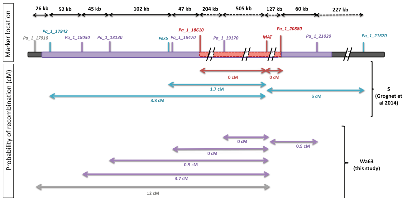
Fig. 6. Probability of recombination in centimorgans (cM) between markers and the mating-type locus in the Podospira anserina heterokaryotic strain Wa63 after several rounds of experimental selfing measured in 109 of the offspring compared with the P. anserina S strain. Relative marker locations compared with the mating-type locus and physical distance (kb) between adjacent markers are shown. Dashed lines indicate regions not represented to scale. The location of the mating-type locus is indicated as “MAT” in red, and the region shown to lack recombination in the P. anserina S strain is indicated as a light red rectangle, with markers located at the margin of the nonrecombining region ( Pa_1_18610 and Pa_1_20880 ) also indicated in red. Frequencies of recombination for the S strain, as inferred with the markers used by Grognet et al. (2014), are indicated in blue. The region with elevated dS in the Wa63 strain before experiment selfing but with zero dS in the S strain is indicated as a purple rectangle. Frequencies of recombination for the Wa63 strain, estimated from the genotypes at the five SNP markers according to the PCR-KASP assay for 84 of the F10 or F11 offspring and whole-genome sequencing data for 25 of the F10 offspring are shown in light purple. Frequencies of recombination with the Pa_1_17910 marker, additional marker estimated from the genotypes obtained by the whole-genome sequencing of 25 of the F10 offspring, are shown in gray.
