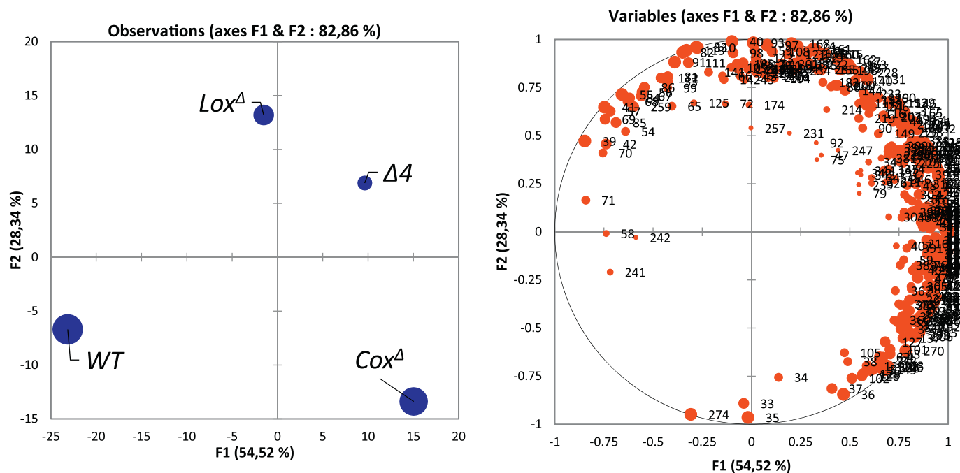
Fig. 1. PCA (left) and associated correlation circle (right) for wild type and mutant strains Cox^{\Delta} , Lox^{\Delta} and \Delta 4 . PCA was constructed from all fragment ions (33 to 425) extracted from the chromatograms, each presenting several hundred peaks. A global volatile chemical print or global emission without a priori was thus determined for each sample. Global emission of each strain is statistically different and specific. Axis 1 clearly separates wild type from mutants.
