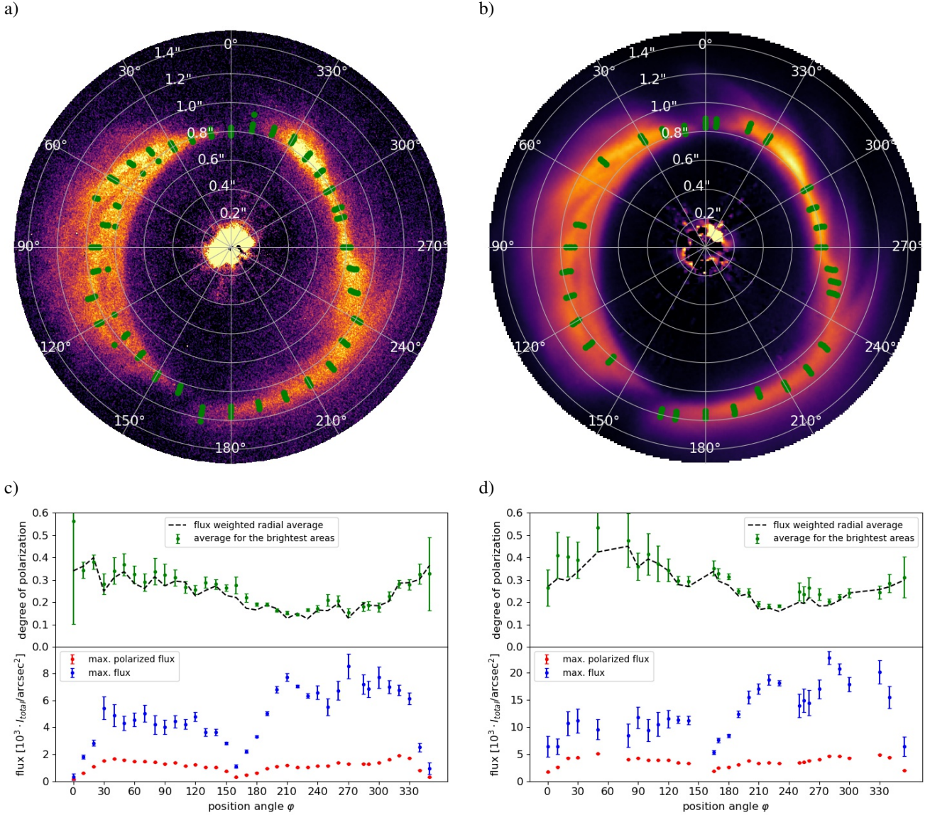
Fig. 9. Polarized intensity of HD 142527 in the VBB (a) and H -band (b) and the corresponding surface brightness \tilde{I}_{\text{disk}}(\phi) , maximum polarized surface brightness \tilde{Q}_{\phi,\text{disk}}(\phi) , and degree of polarization p_{\text{disk}}(\phi) in (c) and (d), respectively. The azimuthal surface brightness profiles in (c) and (d) show the average surface brightness for the four brightest values (indicated by the green dots in (a) and (b)) in each radial profile (see Appendix A). The values are not corrected for signal loss due to PSF smearing. The plots for the azimuthal degree of polarization also show the degree of polarization at the positions where the highest surface brightness was measured (green dots), and additionally show the intensity-weighted average polarization for the complete radial profiles (dashed line).
