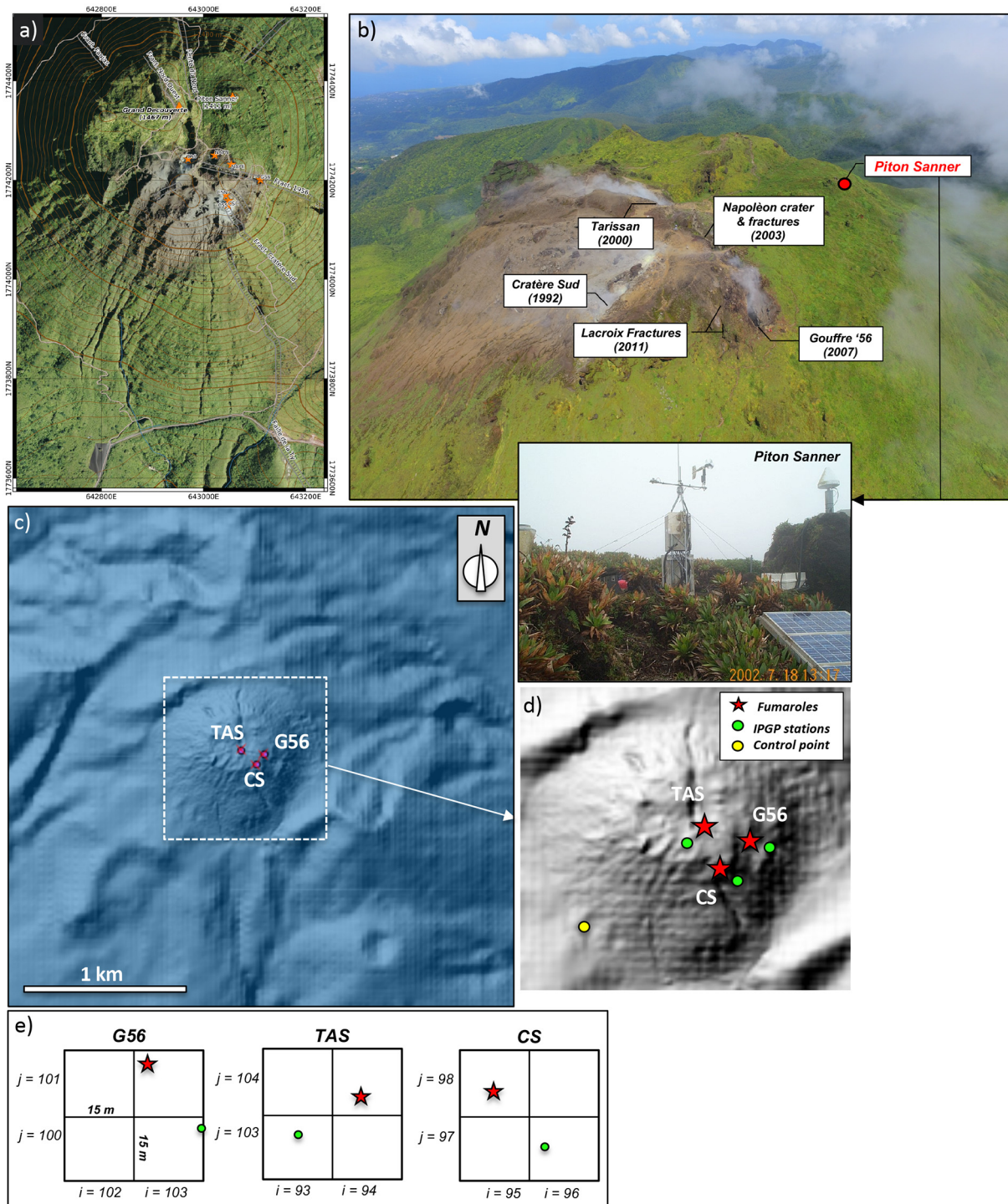
Fig. 1. a) Map of the summit La Soufrière of Guadeloupe volcano (1467 m asl) showing the main geological features (1956 fractures, Cratère Sud, Fente du Nord, Nord-Ovest, Faujas, and La Ty fault), the location of the active fumaroles (red stars) b) photo of the main active fumaroles (Cratère Sud, 1992; Gouffre-56, 2007; Napoléon crater and fractures, 2003; Tarissan, 2000; Lacroix fractures, 2011) modified from Moretti et al., (2020b) and Jessop et al. (2021), and the meteorological station Piton Sanner (1411 m asl); c) Computational domain (ca. 3 km × 3 km) used for numerical simulations. The grid used is set 200 × 200 (resolution = 15 m). The three investigated sources (Cratère Sud, CS; Tarissan, TAS; Gouffre-56, G56) are shown as pink dots; d) Magnification of the summit dome area where are shown the location of the fumarolic sources (red stars; G56: 643531 E, 1774515 N; TAS: 643396 E, 1774549 N; CS: 643481 E, 1774456 N), the IPGP measurement stations (green dots; G56: 643545 E, 1774499 N; TAS: 643388 E, 1774541 N; CS: 643489 E, 1774441 N) and the control point located at the south-western flank (yellow dot; 643,108 E; 1,774,190 N); e) Position of the fumarolic sources (red stars) and stations (tracking points, green dots) on the cells (i,j) of the 15 m-resolution computational grid.
