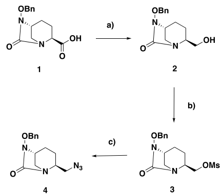
Scheme 2: a) i. \text{CICO}_2\text{iBu} , \text{NEt}_3 , THF, 0^\circ\text{C} , 2h, ii. \text{NaBH}_4 , 0^\circ\text{C} , 3h; b) \text{MsCl} , DMAP, \text{NEt}_3 , DCM, 0^\circ\text{C} , 2h; 3) \text{NaN}_3 , DMF, 90^\circ\text{C} , 20h (35% over 3 steps).
