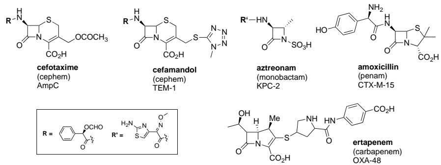
Figure 2. Structure of \beta -lactam antibiotics used as substrates to determine the activity of \beta -lactamases TEM-1, KPC-2, CTX-M-15, AmpC, and OXA-48. The drugs belong to the cephem, monobactam, penam, or carbapenem classes of \beta -lactams, as indicated in parenthesis.
