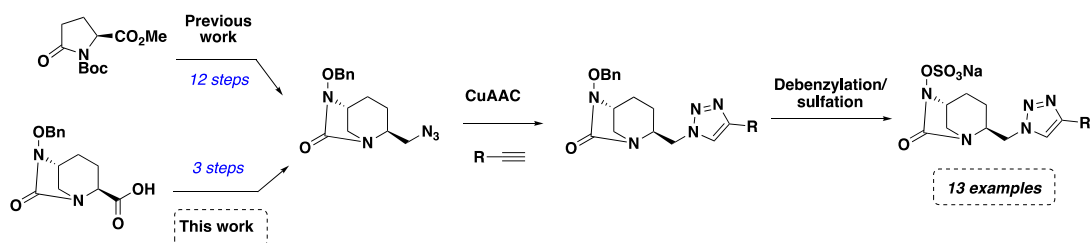
Scheme 1. Strategies to access functionalized DBOs.
