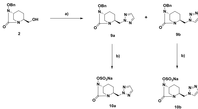
Scheme 5. a) i. MsCl, NEt 3 , DMAP, DCM, 0°C, 1h, ii. 1H-1,2,3-triazole, tBuOK, MeCN, reflux, 15h; 9a (44%); 9b (37%); b) i. Pd/C, H 2 , MeOH, rt, 48h, ii. SO 3 -Pyr, pyridine, rt, overnight, iii. DOWEX Na + ; 10a (27%); 10b (8%).
