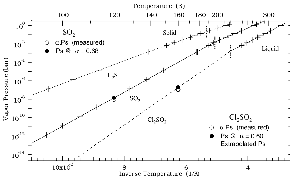
Figure 5. Saturation vapor pressure of H 2 S, SO 2 and Cl 2 SO 2 as a function of temperature. Data for solid and liquid H 2 S and SO 2 (crosses) are from Honig and Hook [1960]. Our sublimation rate measurement of SO 2 ice at 120 K (circle) is consistent with the SO 2 curve with a condensation coefficient \alpha \approx 0.68 \pm 0.15 (dot). Data for liquid Cl 2 SO 2 are from Lide [1990]. The vapor pressure curve of solid Cl 2 SO 2 (dashed line) is obtained by fitting a thermodynamic law to our data at 160 K (dot; assuming \alpha \approx 0.60 ) and to the saturation pressure at the triple point.
