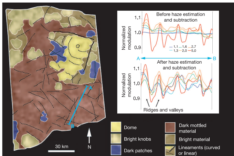
Figure 4 | Geological interpretation of the high-resolution image. On the basis of albedo variations and variations in texture, a geological interpretation of the circular feature has been obtained (left panel). Analysis of I/F variations have been realized along profile A–B. The upper panel and the lower panel on the right shows I/F before and after removal of the haze-scattering effect, respectively. Our interpretation of topography rests on several factors: (1) the highest contrast in the topography is in the cross-sun direction; (2) topographic forms have characteristic bilateral symmetry (bright–dark oscillations in the down-sun direction); and (3) after haze removal at shorter wavelengths, the topographic patterns do not correlate in general with variations in spectral reflectance. In addition to
