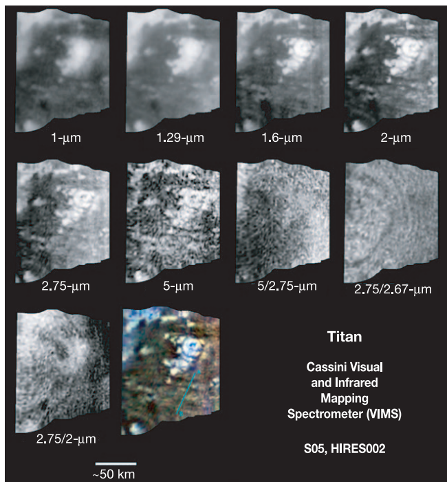
Figure 3 | High-resolution image of Fig. 2d at different wavelengths.
