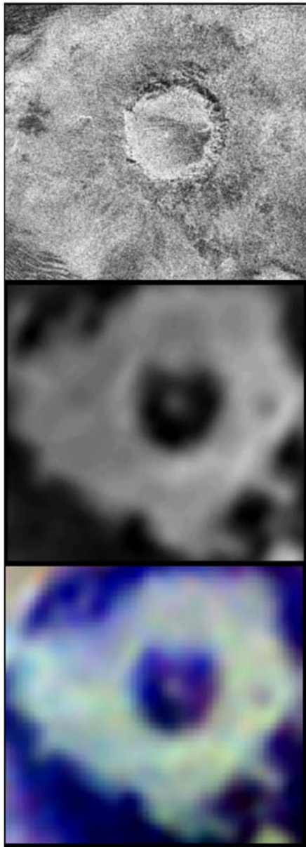
Figure 9. SAR image (top) and VIMS T13 (2- \mu m image in the middle and false color ratio composite at the bottom) images of the Sinlap crater, showing a possible central peak.
