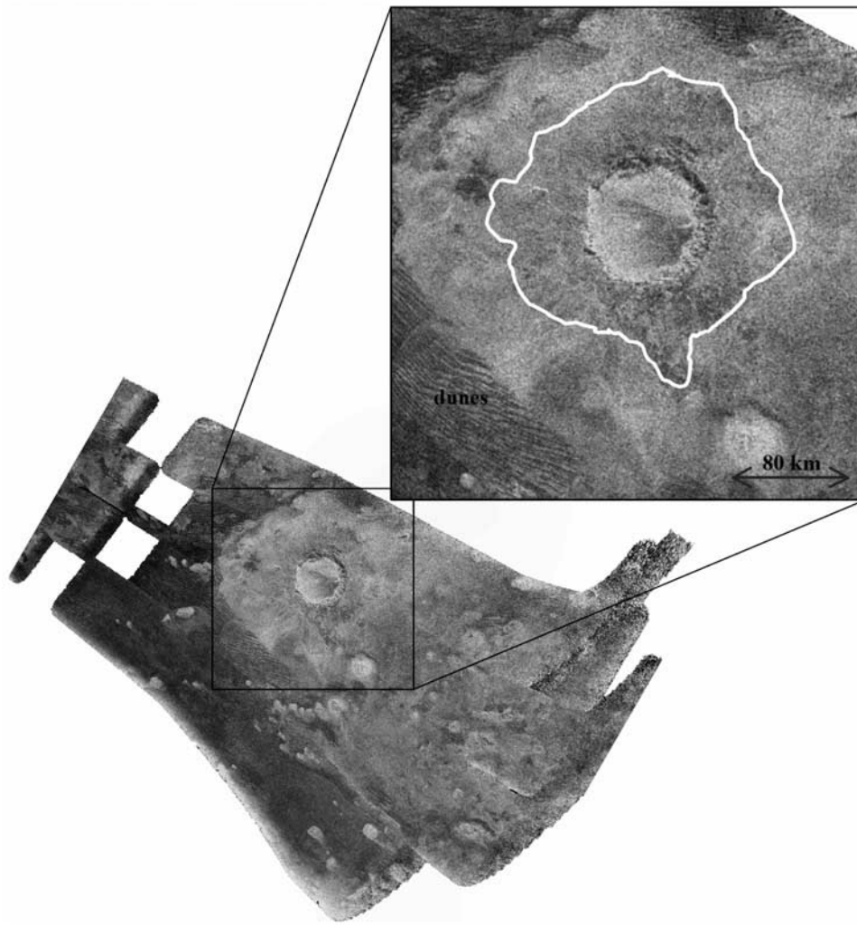
Figure 6. SAR image of Sinlap acquired at T3 on 15 February 2005 and zoom of the crater structure. The white line corresponds to the location of a slightly darker (in radar) area on the external part of the crater wall, with a mean backscatter power of 0.7 dB for an incidence angle varying from 12 to 18 degrees over the scene. It also corresponds to the limits of the bright “ejecta” in VIMS images. The outer radar bright region has a mean backscatter power of 2.4 dB. The SAR image covers an area of \sim 1000 \times 700 km.
