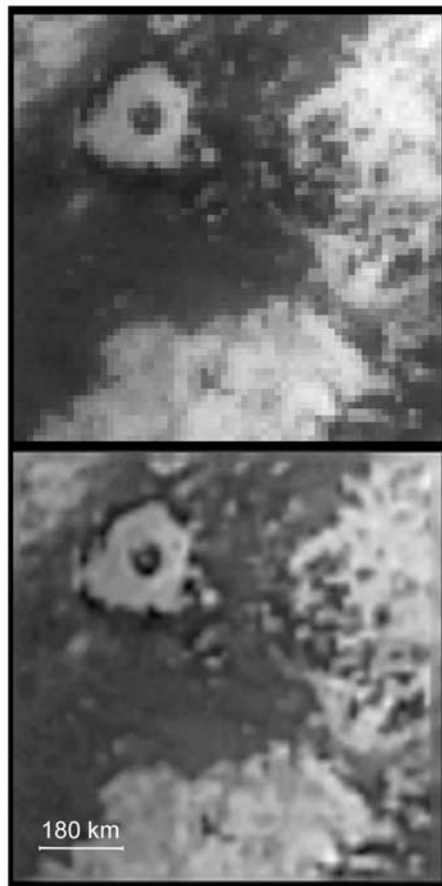
Figure 1. Enhancement of surface features. Top: raw VIMS channel at 2.03\ \mu\text{m} . Bottom: same after co-addition of 12 channels within methane windows, oversampling, bilinear interpolation and unsharp mask procedure. The circular bright feature is named Bazaruto Facula, which surrounds Sinlap crater.
