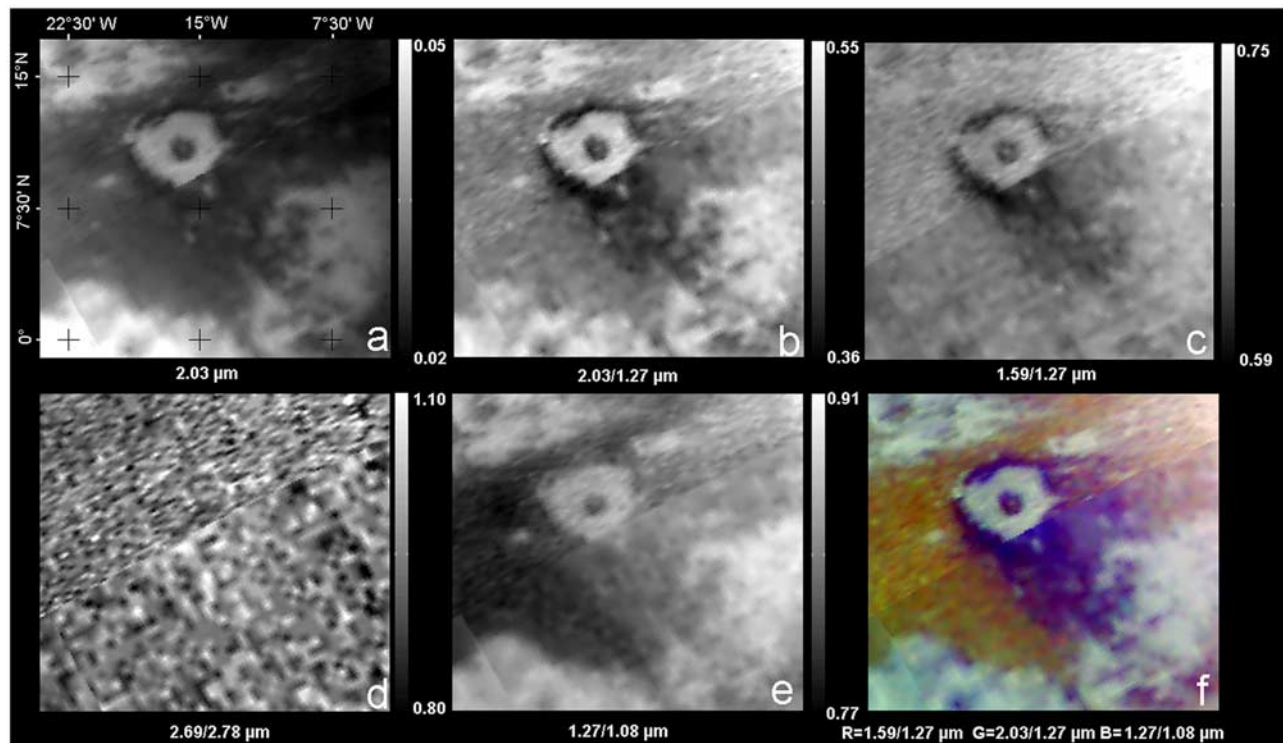
Figure 2. VIMS T5 (16 April 2005) observations of Sinlap, acquired with a spatial resolution of 18 km/pixels and a solar incidence angle from 63^\circ to 84^\circ . (a) 2.03\text{-}\mu\text{m} image, with I/F values ranging from 0.02 to 0.05. (b) to (e): Band ratios. (f): False RGB color composite of band ratios. Sinlap appears as a bright annulus surrounded by an area absorbing at 1.59 and 2.0\text{ }\mu\text{m} (but not at 1.08 and 1.27\text{ }\mu\text{m} ), with a parabolic shape oriented toward the South East.
