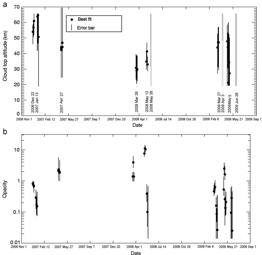
Fig. 4. (a) Cloud altitudes derived from the SPSSDISORT radiative transfer model, computed on several pixels by flyby. The points correspond to the best fit, and the lines to error bars for each point. The clouds are always found at the same altitude range, between 30 and 65 km. The modeling analysis did not allow to derive the altitude for the flybys T44, T52 and T56, probably due to a combined effect of the low spatial resolution and of the progressive decrease of the cloud thickness. (b) Cloud opacities derived from the SPSSDISORT model.
