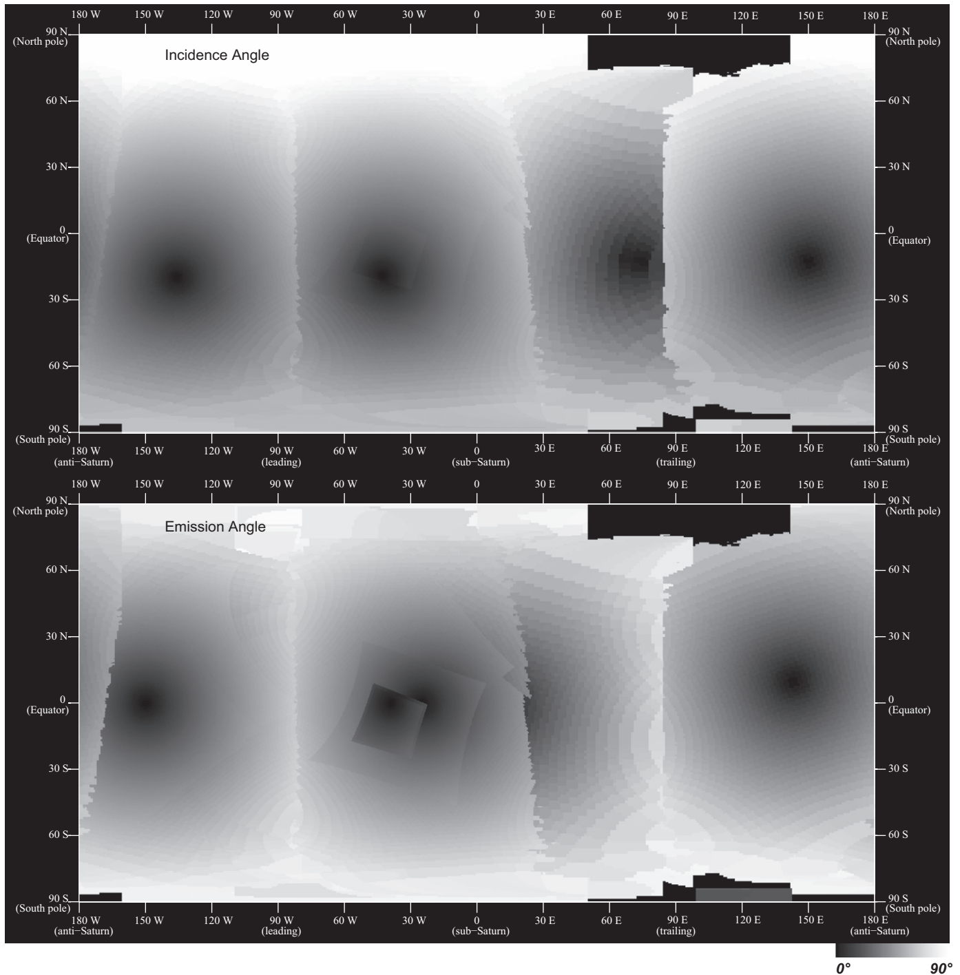
Fig. 5. The top map represents the incidence angle as it changes over each flyby. The bottom map represents the emission angle. The angle, in both cases, build up as we approach the center of a flyby, then starts to drops off. These maps identify the nadir points where the signal-to-noise ratio is the greatest in relation to the resolution in Figs. 3 and 6.
