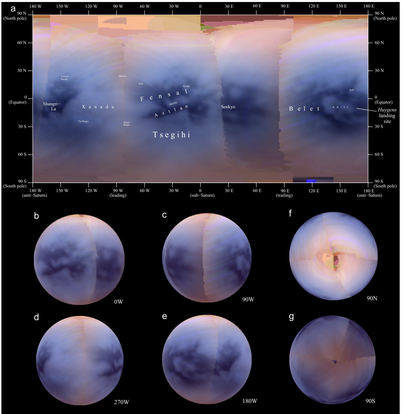
Fig. 6. This is a corrected global map of Titan, using the same color/wavelength scheme as Fig. 3, created using an algorithm to divide the haze out of the picture. In doing so, the surface features of Titan become more pronounced. Removing some of the haze also brings out the striping effects that are inherent to the VIMS-V system. When compared to Fig. 3, we can see new areas emerge, such as the section south of Shangri-La in the west.
