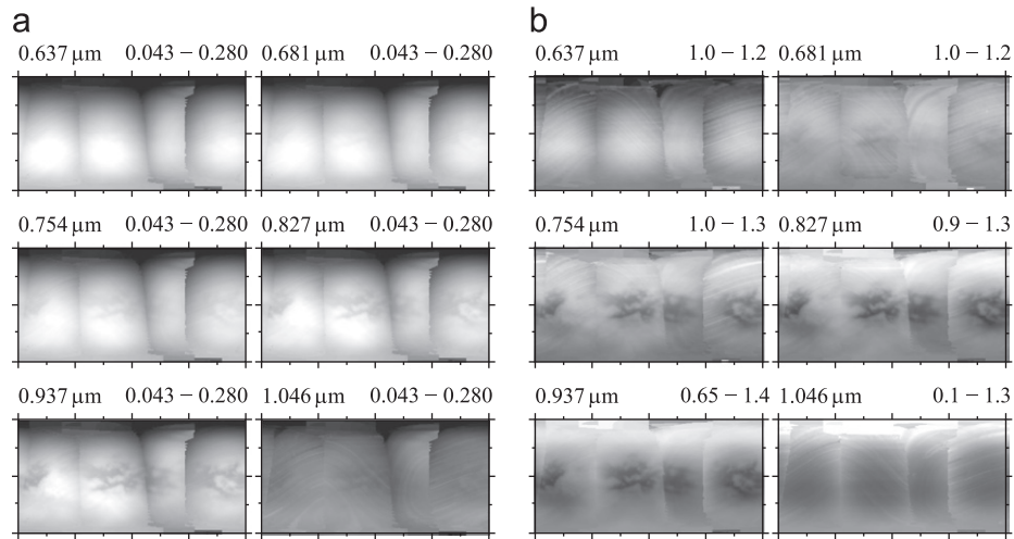
Fig. 2. On the left are I/F maps of Titan without atmospheric correction. Wavelength and contrast are listed in the top left and top right, respectively, of each image. On the right are corrected maps, with the haze divided out according to the Perry et al. (2005) empirical algorithm described in the text. Contrast is constant in the left set of images and set to maximize surface feature distinction in the right.
