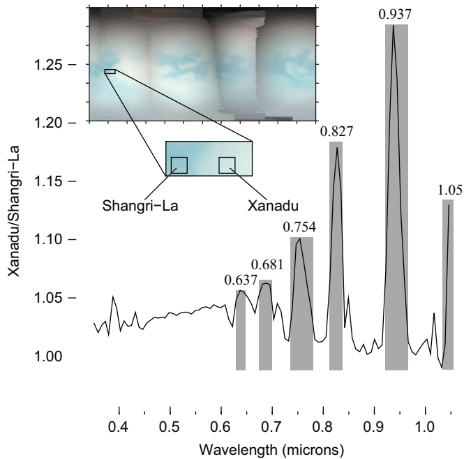
Fig. 7. A spectral ratio graph, created using the T8 flyby, depicting the detected flux from a bright area relative to that in a dark area. It represents the average value of Xanadu divided by Shangri-La versus wavelength in microns with optical wavelength windows labeled and the range of the windows boxed. At wavelengths with strong atmospheric absorption, the flux coming from Xanadu and that from Shangri-La are about the same, barring a small difference owing to different haze reflections resulting from view geometry. Within spectral windows, where there is little or no methane absorption, the much higher surface reflectivity of Xanadu results in higher ratios. The ratio for longer-wavelength windows is progressively higher than that for shorter-wavelength windows because the ratio is less affected by scattering off of haze particles. Windows exist at 0.637, 0.681, 0.754, 0.827, 0.937, and 1.05 \mu\text{m} .
