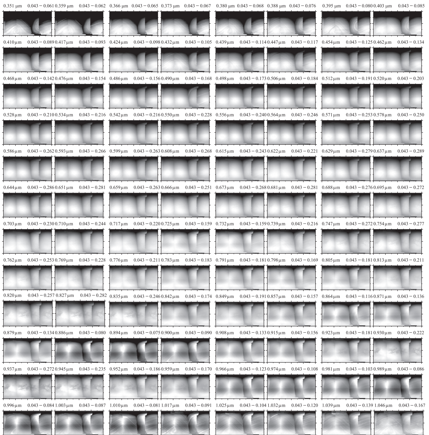
Fig. 1. The top left window represents the beginning of the wavelength range of Cassini VIMS' 96 optical wavelength channels, 0.35 μm, and wavelength increases for each row. A quick look over all of the different wavelengths in the figure above reveal that there are few that show the surface. Methane has fewer windows in the optical spectrum than it does in the infrared, and scattering is more prevalent, but we can still see distinctions on Titan's surface.
