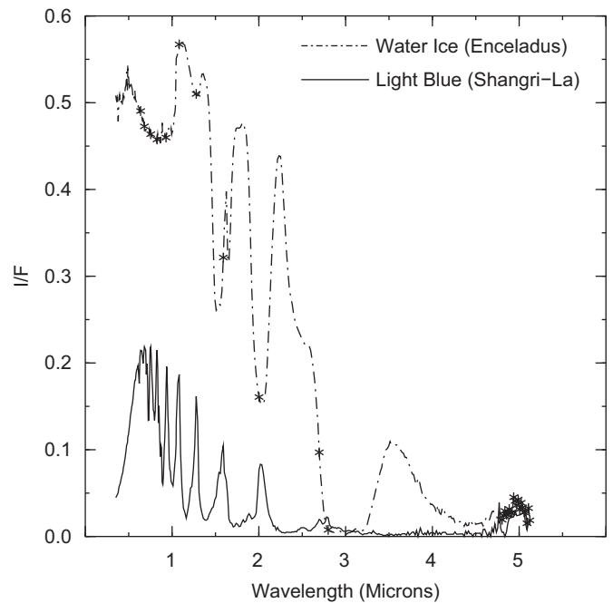
Fig. 9. A comparison between water ice (for reference) and the visible light blue spectral type taken from northern Shangri-La. The stars in the Enceladus line represent the atmospheric windows in both the visible and IR. The overall gray appearance and greater relative brightness compared to the IR in the visible wavelengths in the Titan spectrum is broadly consistent with water ice, and also with various organic materials. Inversions from minima to maxima in these graphs imply wavelengths where a signal may be transmitted without being absorbed.
