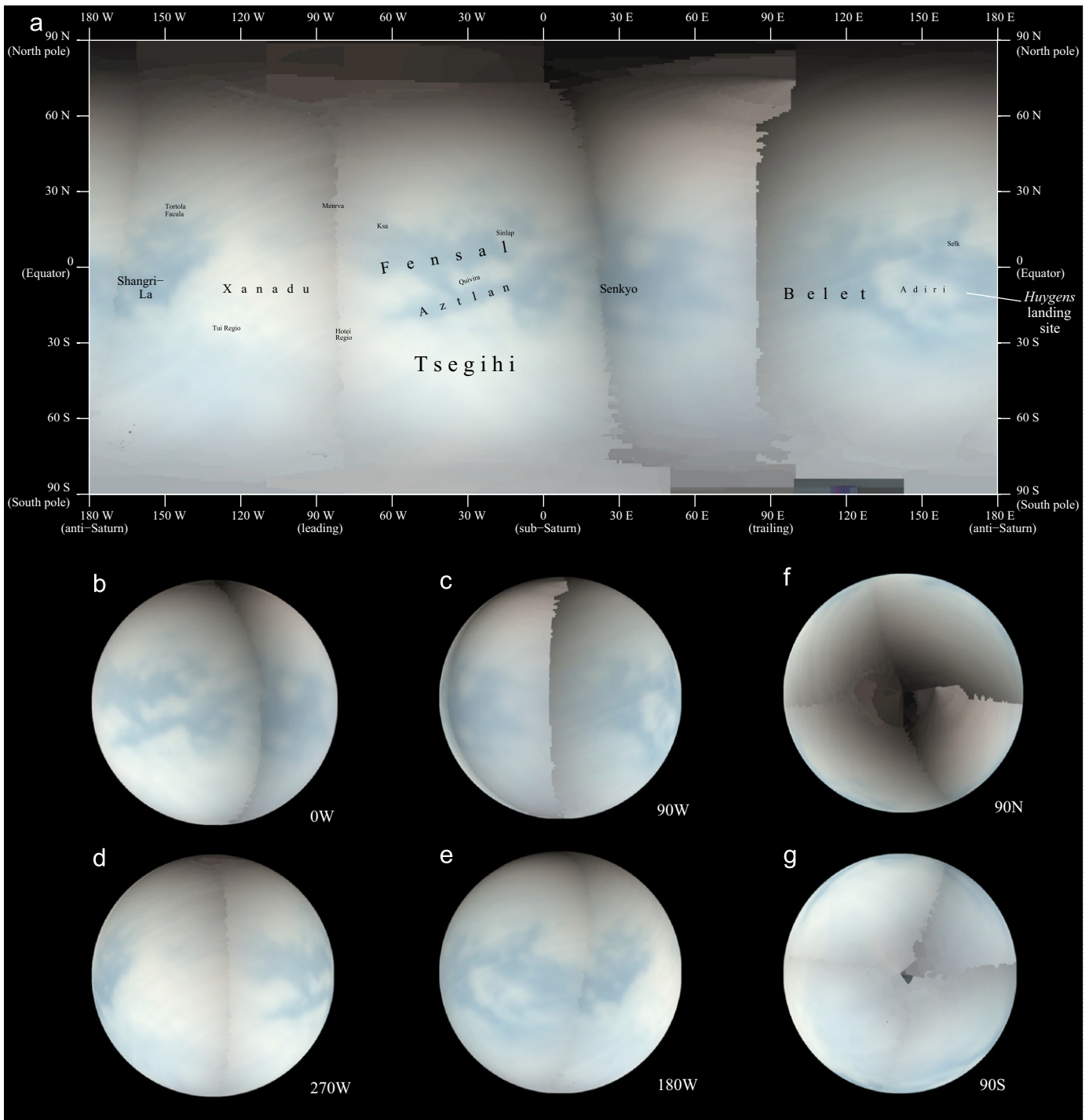
Fig. 3. The atmospherically uncorrected I/F map of Titan shown is made via VIMS from T8, T9, T31, T34, and rev9 in cylindrical projection (a). The colors and wavelengths used to make this map are red at 0.937 \mu\text{m} , green at 0.827 \mu\text{m} , and blue at 0.754 \mu\text{m} . Part a of the figure shows a simple cylindrical map of the five flybys sewn together. Parts b–g of the figure show the different faces of Titan in an orthographical projection. In comparison to infrared maps, our optical map shows less distinction between different wavelengths. However, note that the 5\text{-}\mu\text{m} bright spots do not stand out with the exception of Tui Regio. (For interpretation of the references to color in this figure legend, the reader is referred to the web version of this article.)
