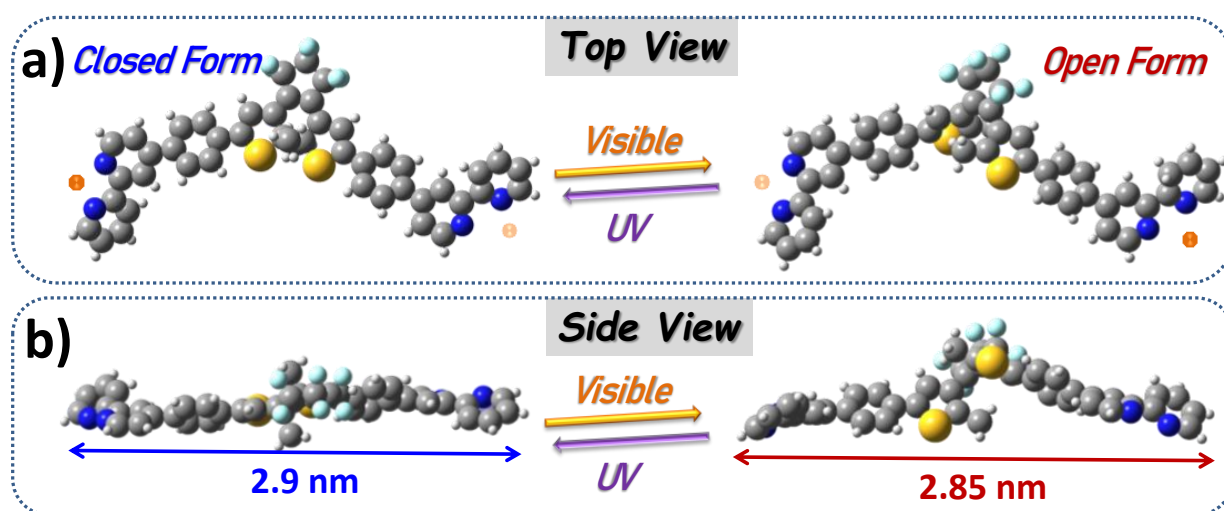
Scheme 1. Top (a) and side (b) views of bpy-DAE-bpy CF and OF isomers switchable by UV-Visible light irradiation. Molecular lengths are calculated. Gray, blue, yellow and white balls represent C, N, S and H, respectively. Orange balls represent H^+ ions.
