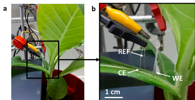
Fig. 2. (a) Electrochemical cell used for in vivo measurements; (b) enlarged picture of the cell.
