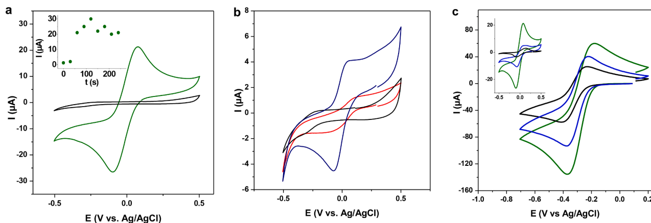
Fig 3. CVs acquired in a plant leaf treated with 30 mM \text{K}_3\text{Fe}(\text{CN})_6 : (a) (green) through immersion (inset: current at 0 V as a function of time of immersion in the uptake solution); (b) (blue) injection of 25 \mu\text{L} of solution and (red) agro-infiltration of 100 \mu\text{L} of solution; CV in untreated leaves are shown in black. (c) CVs acquired in the plant after 3 h immersion in 30 mM \text{Ru}(\text{NH}_3)_6^{3+} or (inset) \text{Fe}(\text{CN})_6^{3-} solution, at various distances from the uptake point: 2 cm (green), 12.5 cm (blue), and 16 cm (dark). Scan rate v = 100 \text{ mV.s}^{-1} .
