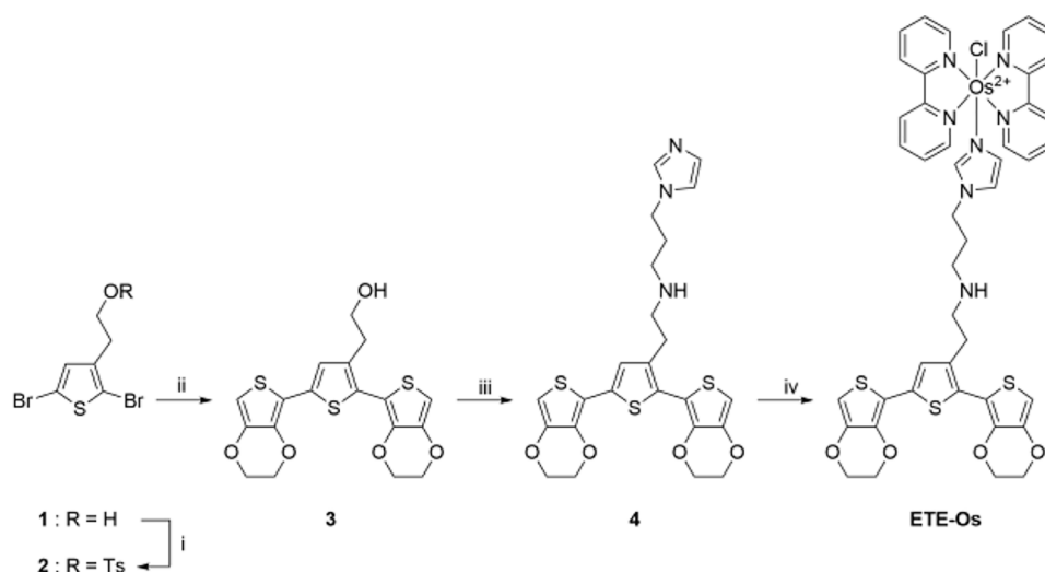
Fig.1. Synthesis of [Os(2,2'-bipyridine)(1-(3-aminopropyl)-imidazole ETE)Cl], ETE-OS . (i):TsCl, pyridine, CH 3 CN, (68%); (ii) EDOT-2-boronic acid pinacol ester, PEPPSI-IPr Pd catalyst, KF, THF/H 2 O (68%); (iii) 1-(3-aminopropyl)-imidazole, CH 3 CN (62%); (iv) [Os(2,2'-bipyridine) 2 Cl 2 ], ethylene glycol, microwave 180 °C.
