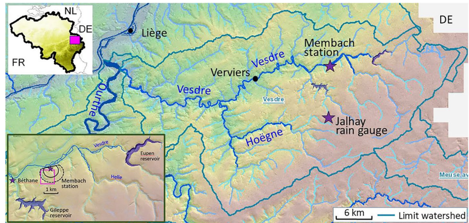
Figure 1. (a) The Vesdre watershed (702 km 2 ) and (b) enlarged view around the Membach station, with the Gileppe and Eupen reservoirs, the Béthane hamlet and the Jalhay rain gauge. The water mass in the areas circled in black contributes 90% (solid line) and 95% (dotted line) of the gravity signal as monitored by the gravimeter. The purple square represents the footprint of the weather radar. Maps from Walloon Geoportail https://geoportail.wallon.be/walonmap .
