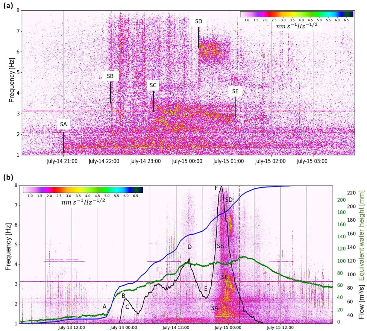
Figure 2. (a) From July 14 20 hr to July 15 4 hr, 2021 Coordinated Universal Time (UTC): moving window spectrum of the recording of the vertical broadband seismometer at the Membach station. The persistent signal around 3.12 Hz is typical of that station, its origin is unknown. (b) From July 13 18 hr to 16, 00 hr, 2021: moving window spectrum of the seismometer, radar-gauge rainfall (blue) and equivalent water height (green), inferred from gravity change by using an admittance of -0.39 \text{ nm/s}^2/\text{mm} (Delobbe et al., 2019). The green scale on the right-hand axis refers to both the precipitation and gravimeter measurements. In black, the inflow in the Eupen reservoir and the vertical dashed line indicates the time at which the flow meter of Verviers, the nearest one, 14 km downstream (distance along the river), broke down. There is an increase in seismic noise during working hours, due to anthropogenic activities, to which is added the rising noise on July 14 caused by the flooding river. Time in UTC.
