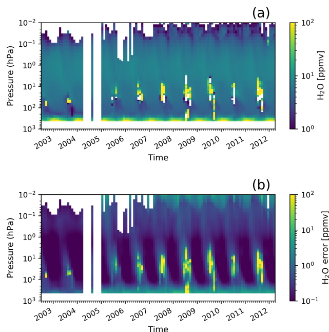
Figure 17. (a) Time series of \text{H}_2\text{O} monthly mean profiles in the latitude belt from 60 to 90° S and (b) corresponding random error when using a CI threshold of 1.8.
