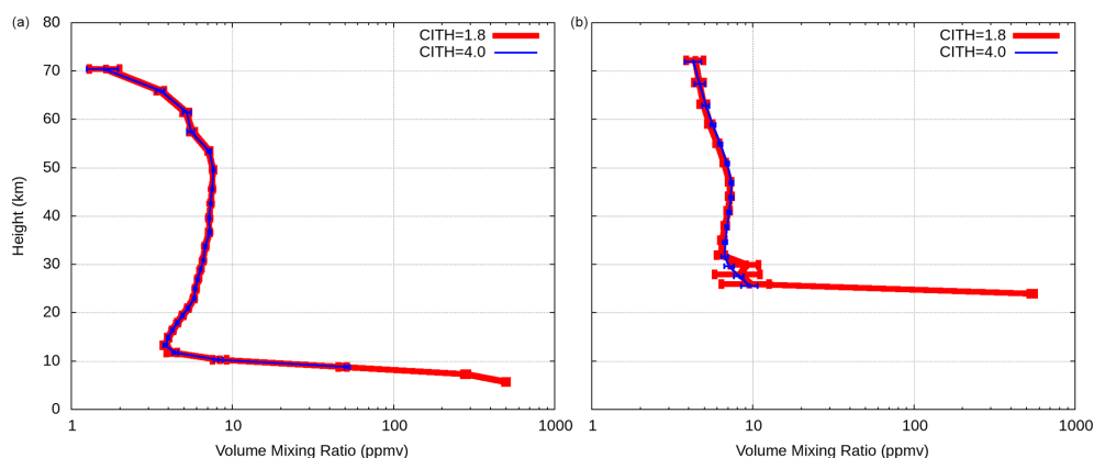
Figure 19. Water vapour profiles retrieved from scan 22 (a, 63^{\circ} N) and scan 71 (b, 61^{\circ} S) of orbit 33153 from 3 July 2008. Red profiles are retrieved after filtering the measurements with a CI threshold of 1.8, the blue profiles with a CI threshold of 4.0.
