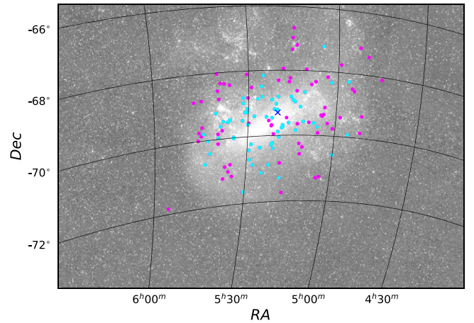
Figure 12. Positions of T2Ceps in the Large Magellanic Cloud considered in this study. Cyan points mark stars observed by the IRSF solely, while magenta points are stars present both in IRSF and VMC catalogs.
