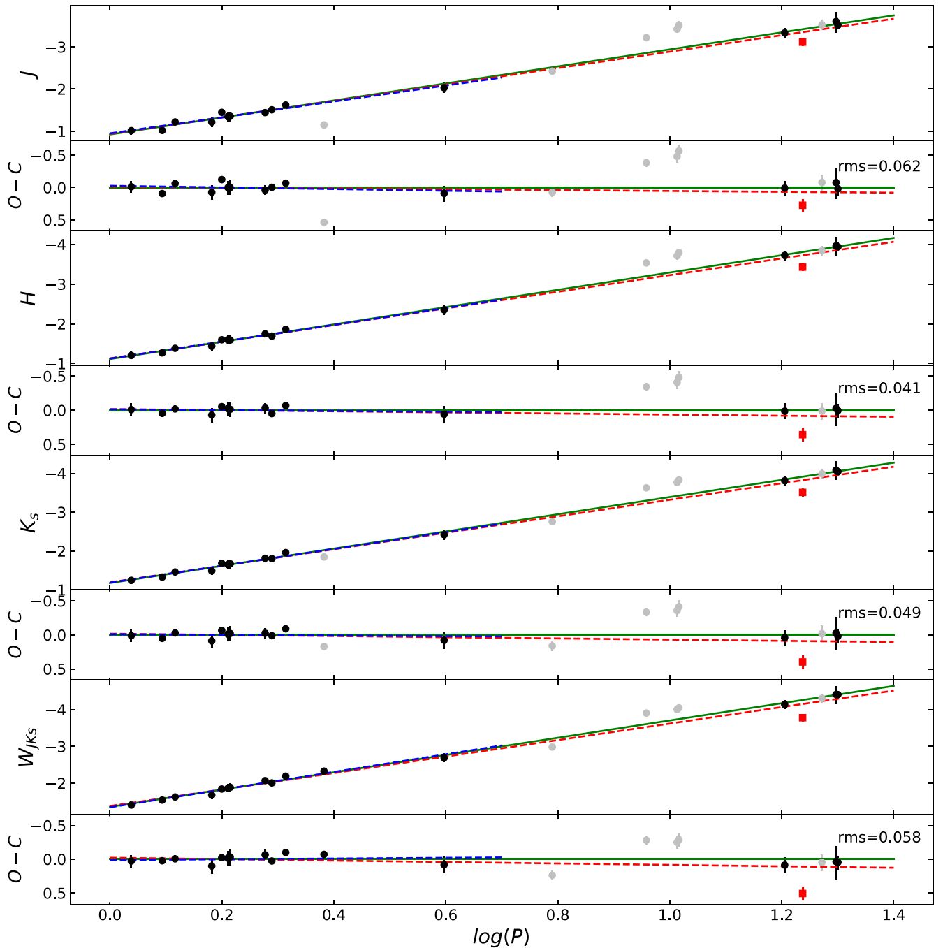
Figure 15. Absolute mean magnitudes of Milky Way T2Ceps in J , H , and K_s and W_{JKs} wesenheit index plotted against logarithm of periods. Black and gray points mark stars used and excluded from fitting procedure, respectively. The red square is W Virginis star, and the red line represent fit including this star, while the green line is obtained excluding it. The blue line is obtained based on BL Her type stars solely. O-C plots present deviations from respective green lines.
