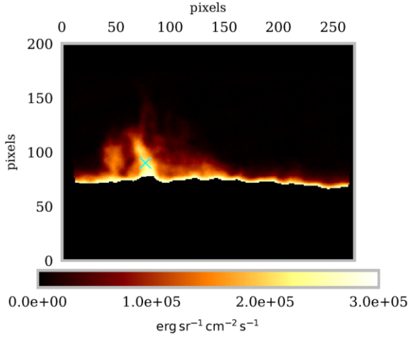
Figure 2. Prominence observed in H\alpha integrated intensity by the MSDP spectrograph. The cyan cross marks the centre of the prominence, where E(H\alpha) \approx 2.2 \times 10^5 \text{ erg sr}^{-1} \text{ cm}^{-2} \text{ s}^{-1} .
