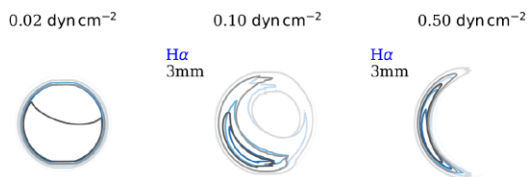
Figure 6. Contour maps for contribution functions for H \alpha compared to the continuum at 3 mm, for multi-thermal prominence models at different pressures. The LOS is directed such that the observer is to the left of each cylinder. The blue contours show H \alpha while the black contours describe the mm-continuum. The contour levels from light to dark correspond to 20, 40, 60, 80, 100 per cent of the maximum of the contribution function in the model prominence.
