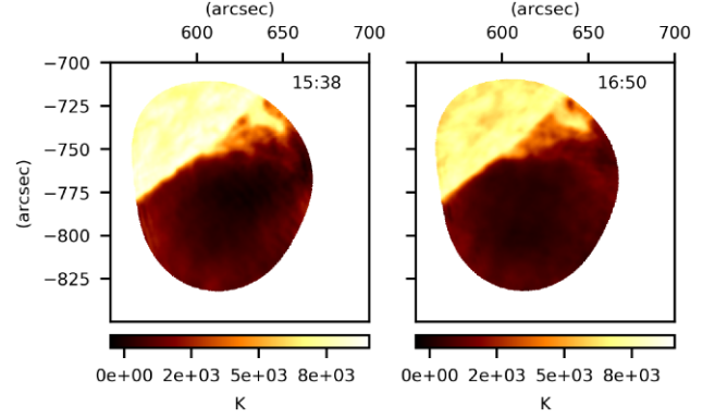
Figure 4. Absolute brightness temperature images of the prominence observed with ALMA Band 3 on 2018 April 19.
